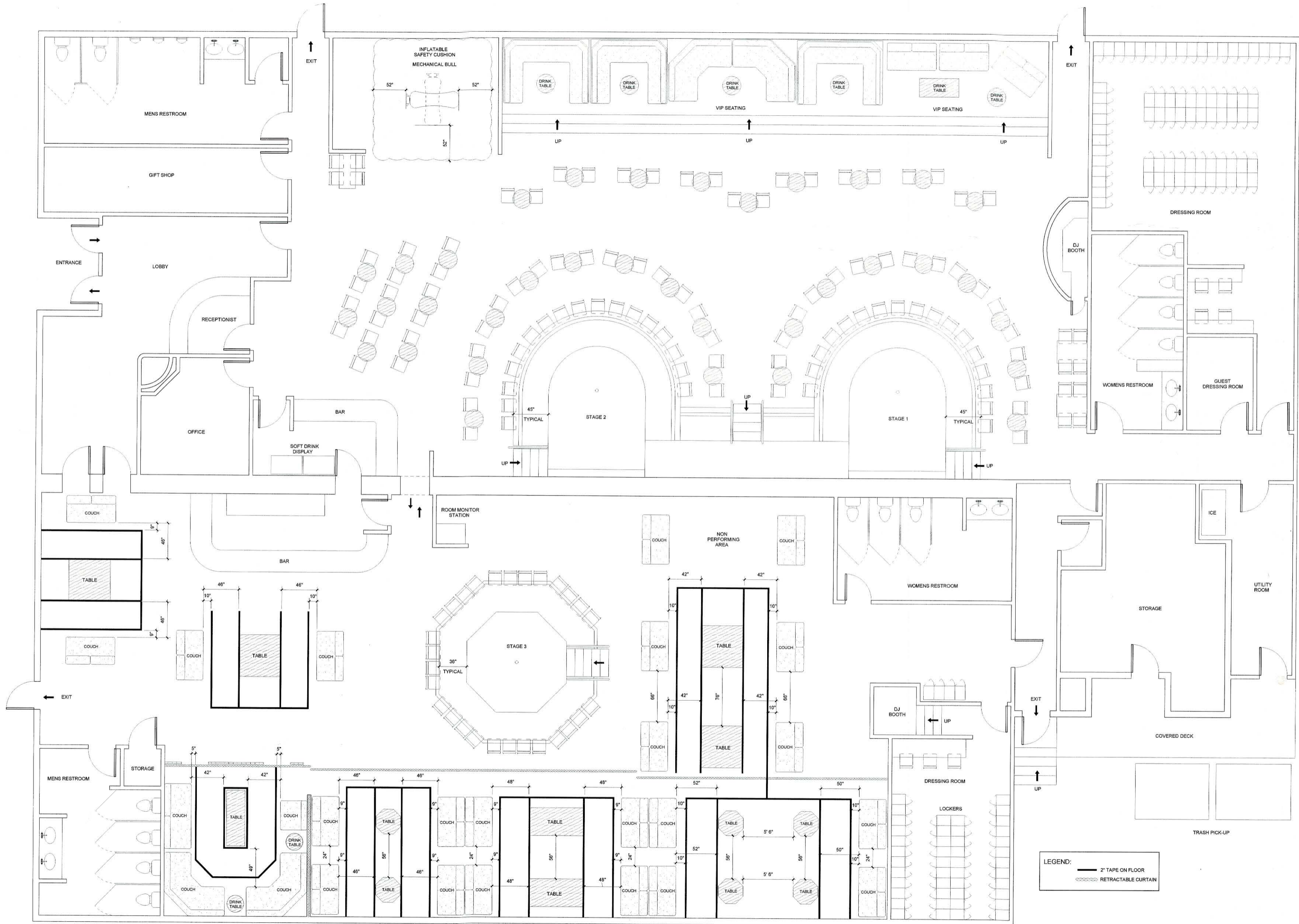
① OPERATIONAL AREAS & ELEMENTS 1/4" = 1'-0"
