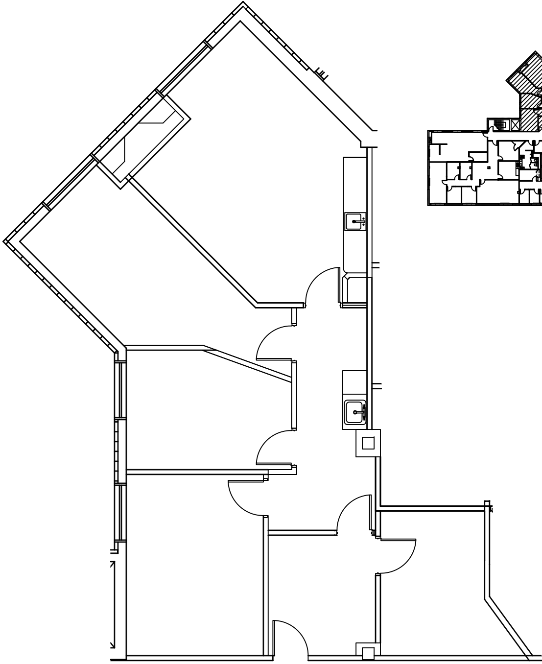
SUITE 440 - FLOOR PLAN 1/8" = 1'-0"
