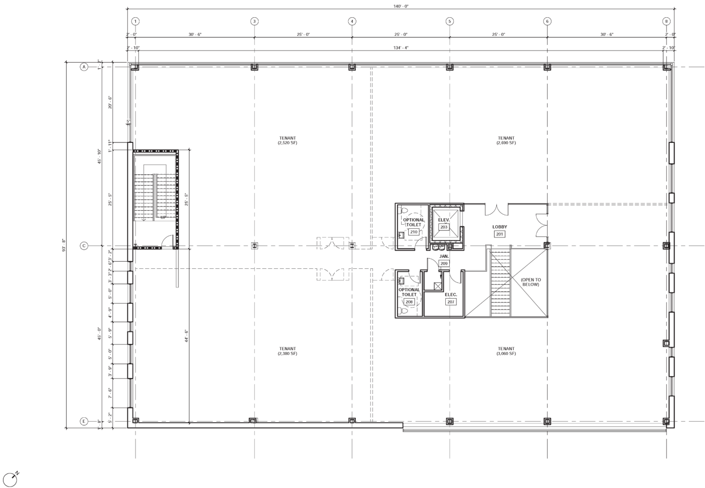
SECOND FLOOR SPACE PLAN
