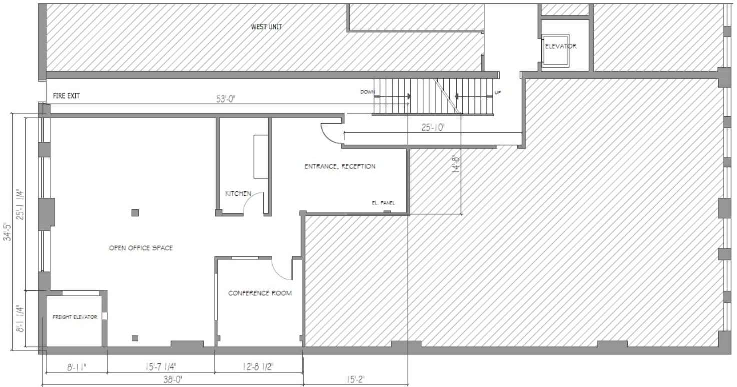
3SE FLOOR PLAN
