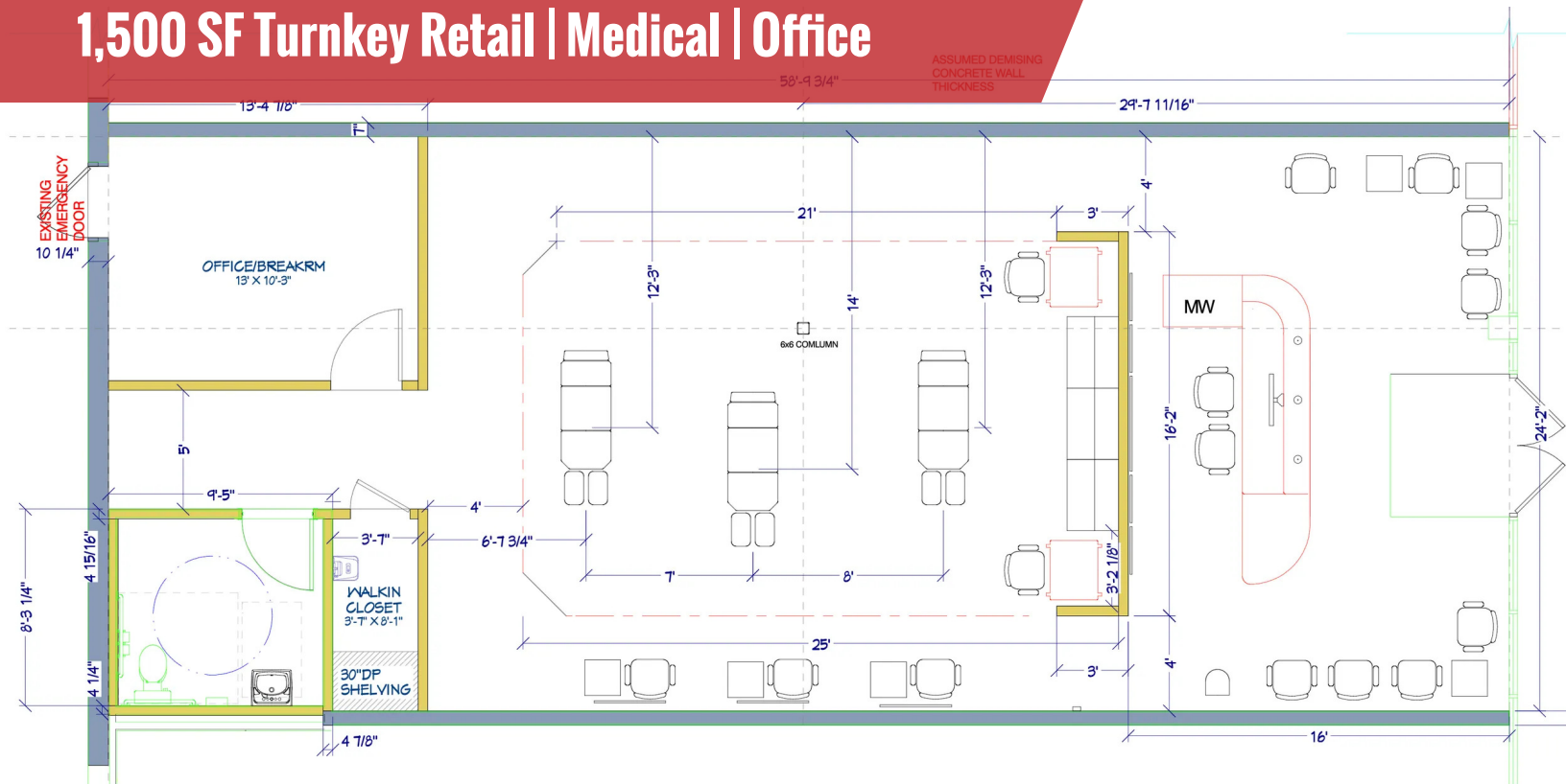
Site Plan
