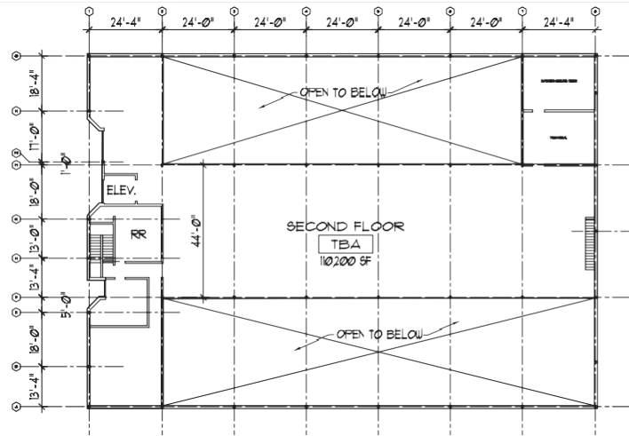
2 SECOND LEVEL SCALE 1/8\"/>
