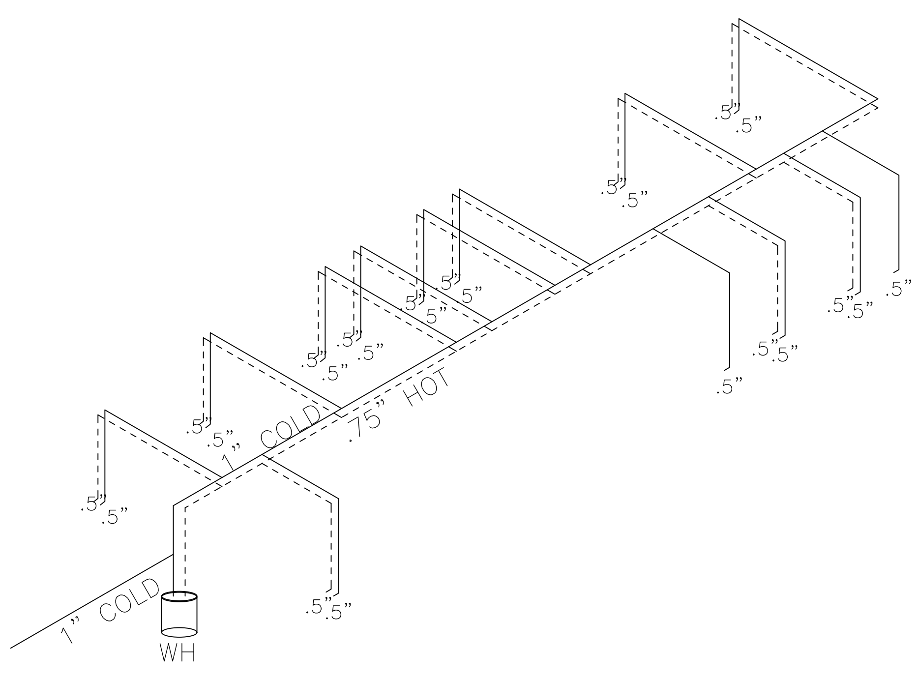
WATER RISER DIAGRAM NOT TO SCALE
