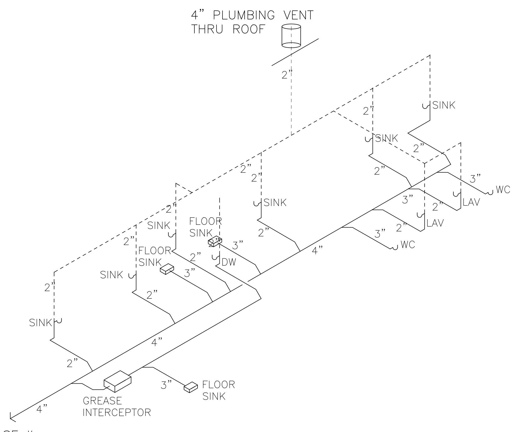
PLUMBING RISER DIAGRAM NOT TO SCALE
