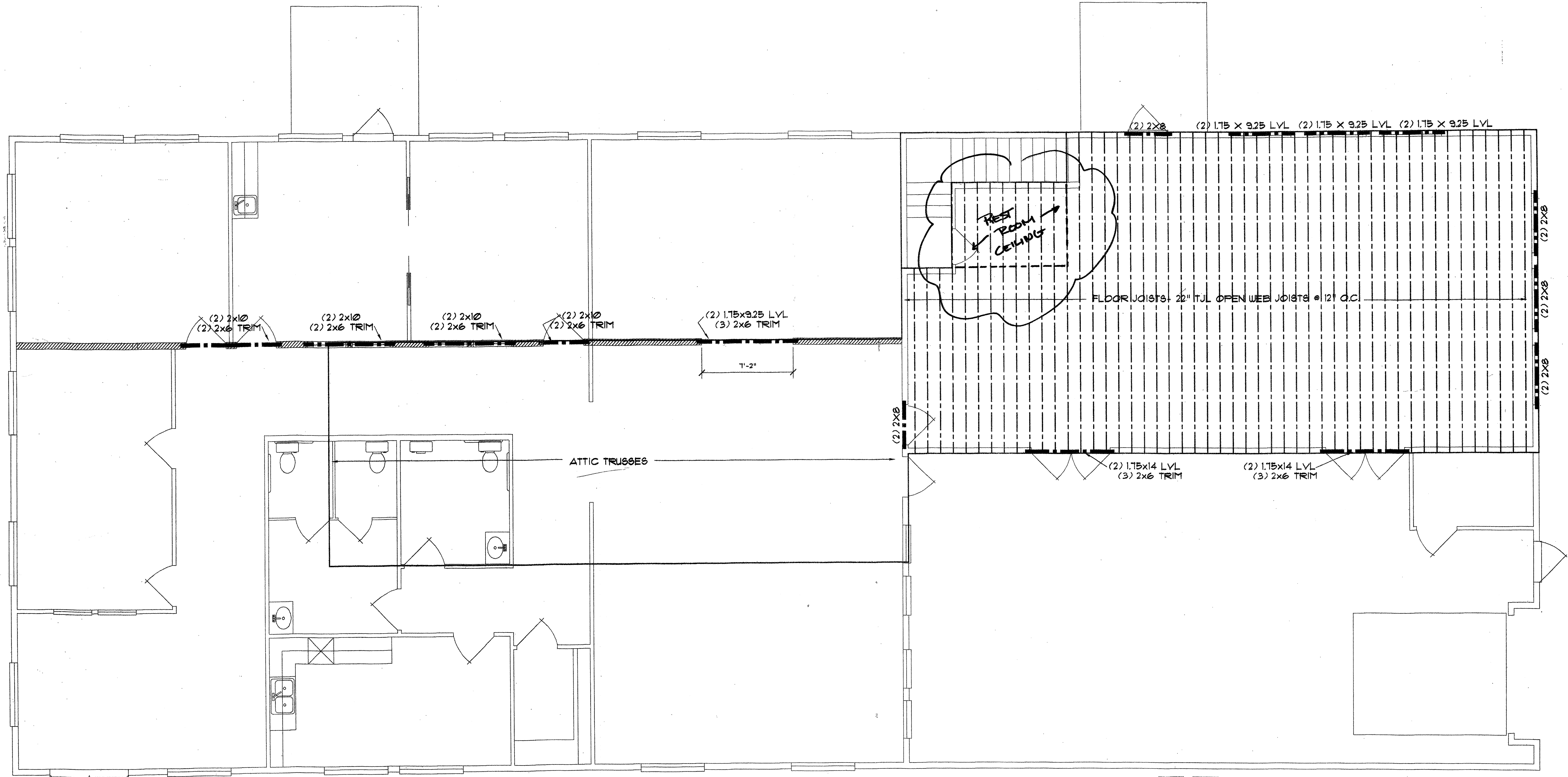
UPPER FLOOR FRAMING PLAN 1/4"=1'-0"
