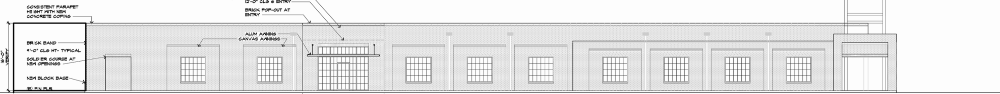
PROPOSED EAST ELEVATION 1/8"=1'-0"
