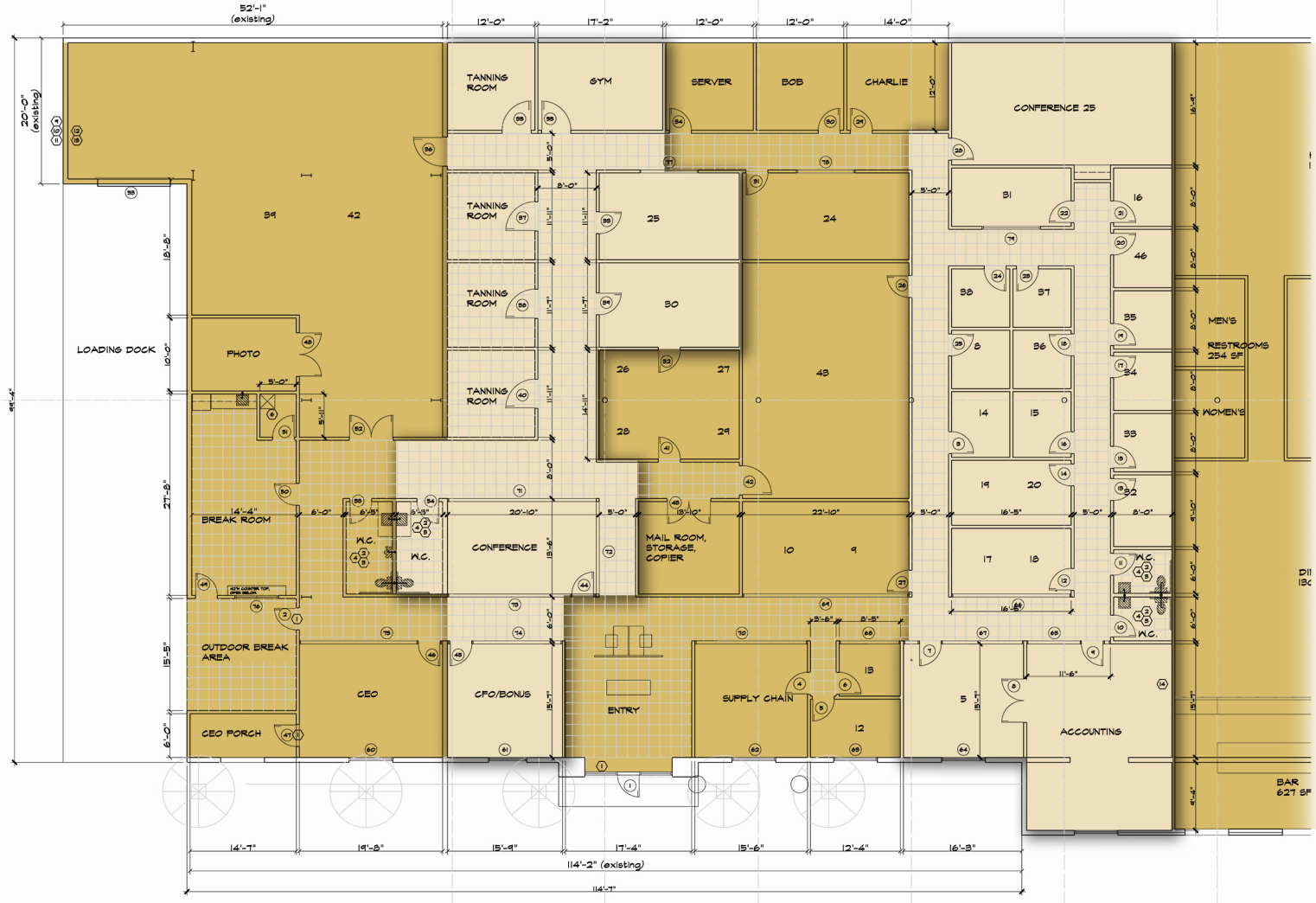
PROPOSED FLOOR PLAN 1/8"=1'-0"
