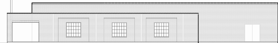
SCHEMATIC NORTH ELEVATION 1/8"=1'-0"
