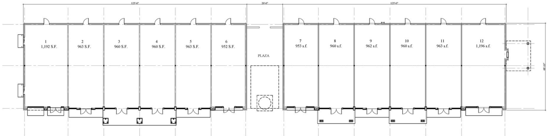
PLAN VIEW BUILDING 1 BUILDING 2
