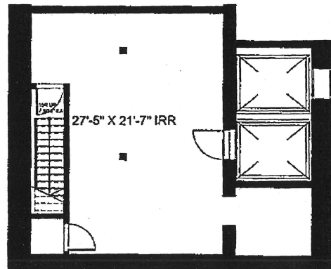
CELLAR FLOOR-STORAGE
