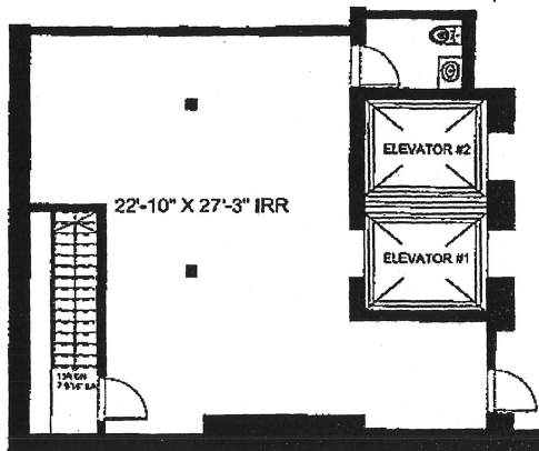
FIRST FLOOR-RETAIL
