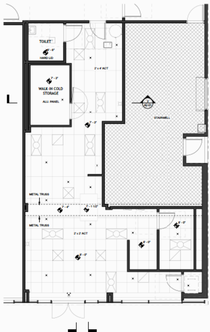
1 REFLECTED CEILING PLAN 1/4" = 1'-0"
