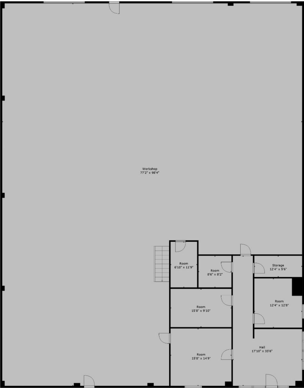
Floor 1
