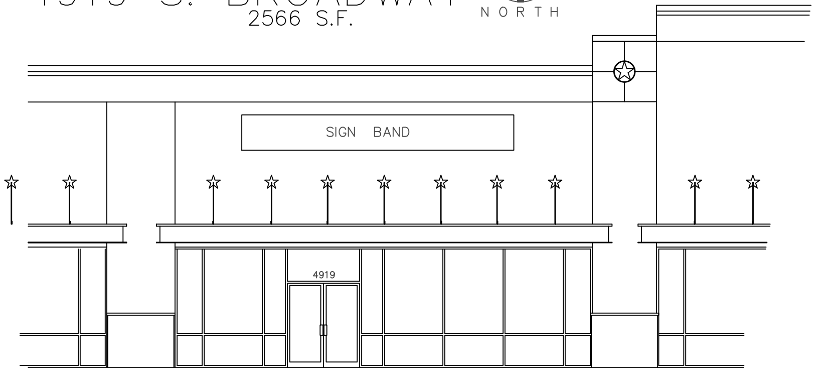
SOUTH ELEVATION
