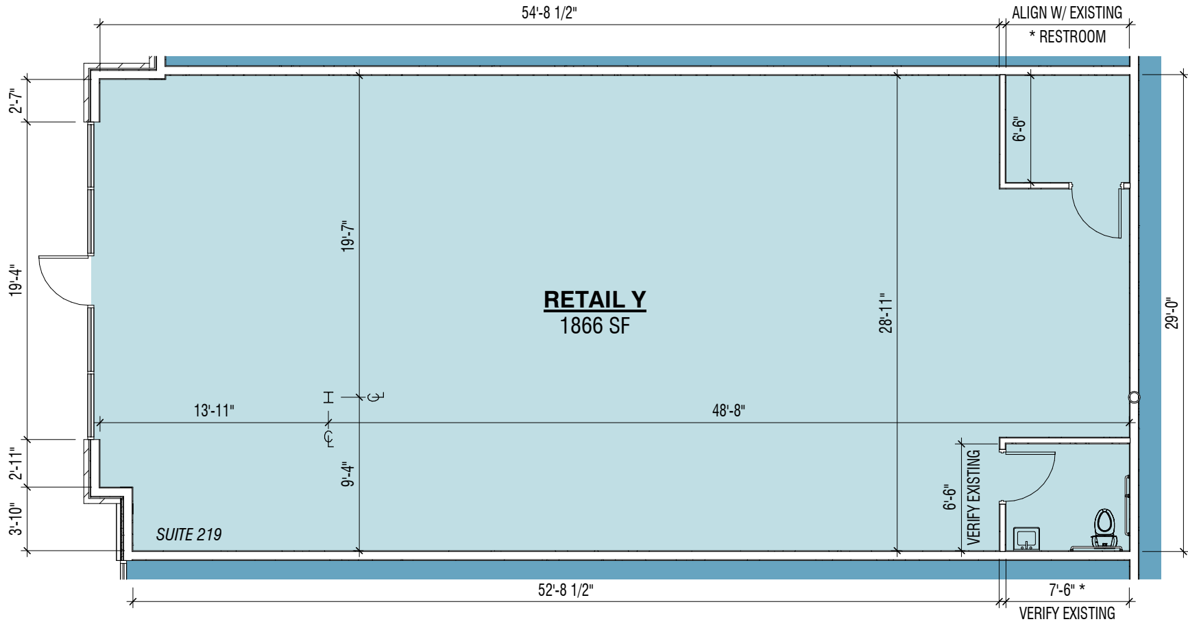
1 01 FIRST FLOOR AREA PLAN (RENTABLE) - SUITE 219 - RETAIL Y SCALE: 1/8" = 1'-0"
