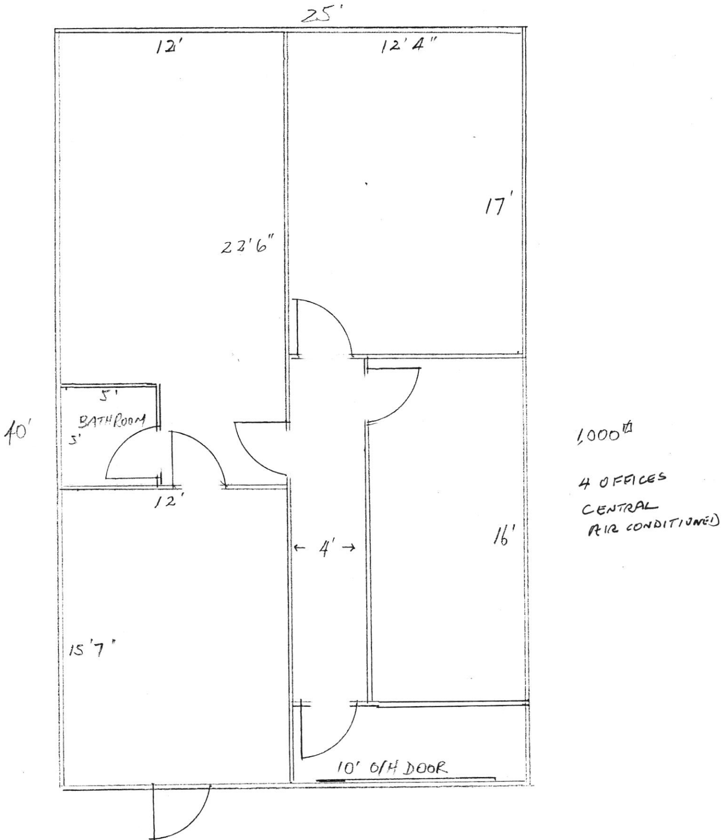
FLOOR PLAN SUITE 220 4531 AYERS ST CORPUS CHRISTI TX
