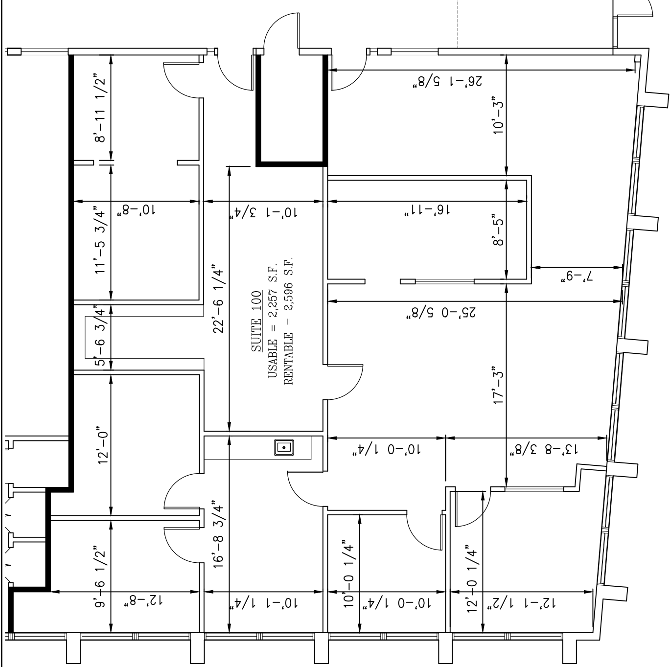
1 SUITE 100 FLOOR PLAN
