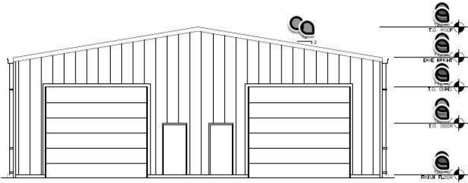
3 REAR EXTERIOR ELEVATION SCALE: 3/16" = 1'-0"
