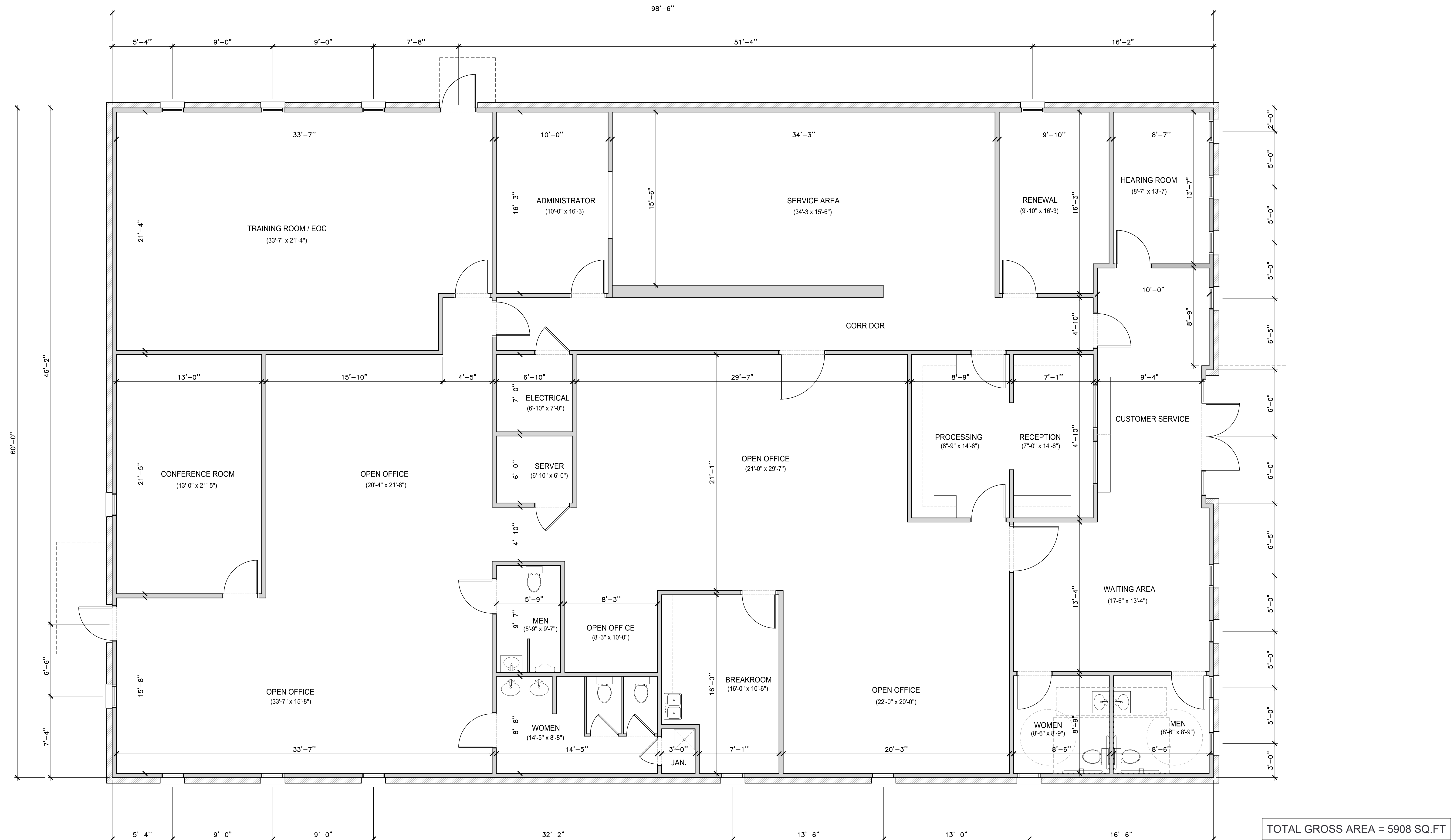
FLOOR PLAN (AS BUILT) SCALE: 1/4" = 1'-0"
