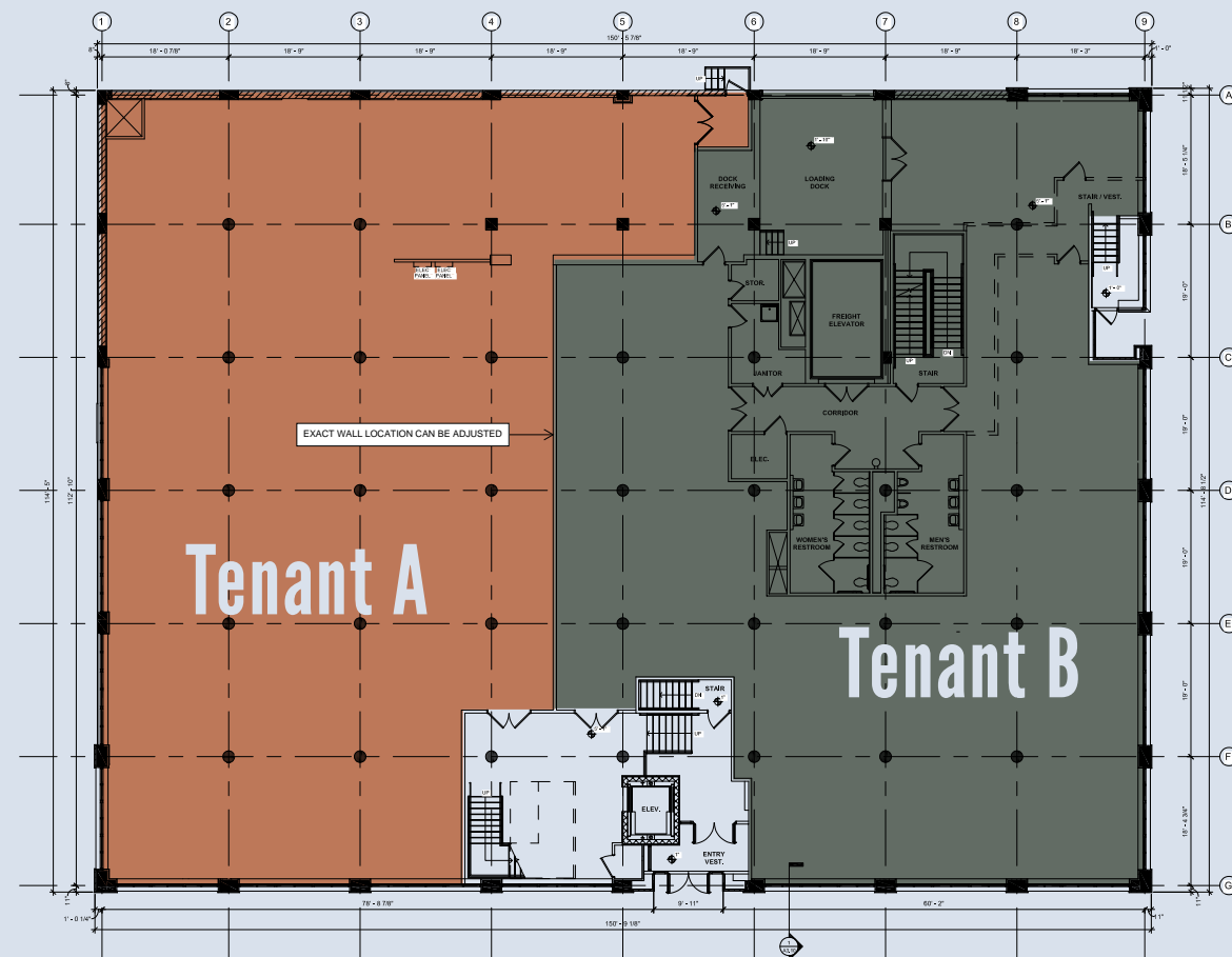
LEVEL 1 FLOOR PLAN - TWO LEVEL 1 TENANTS - LOBBY ENTRIES SCALE: 1/16" = 1'-0"
