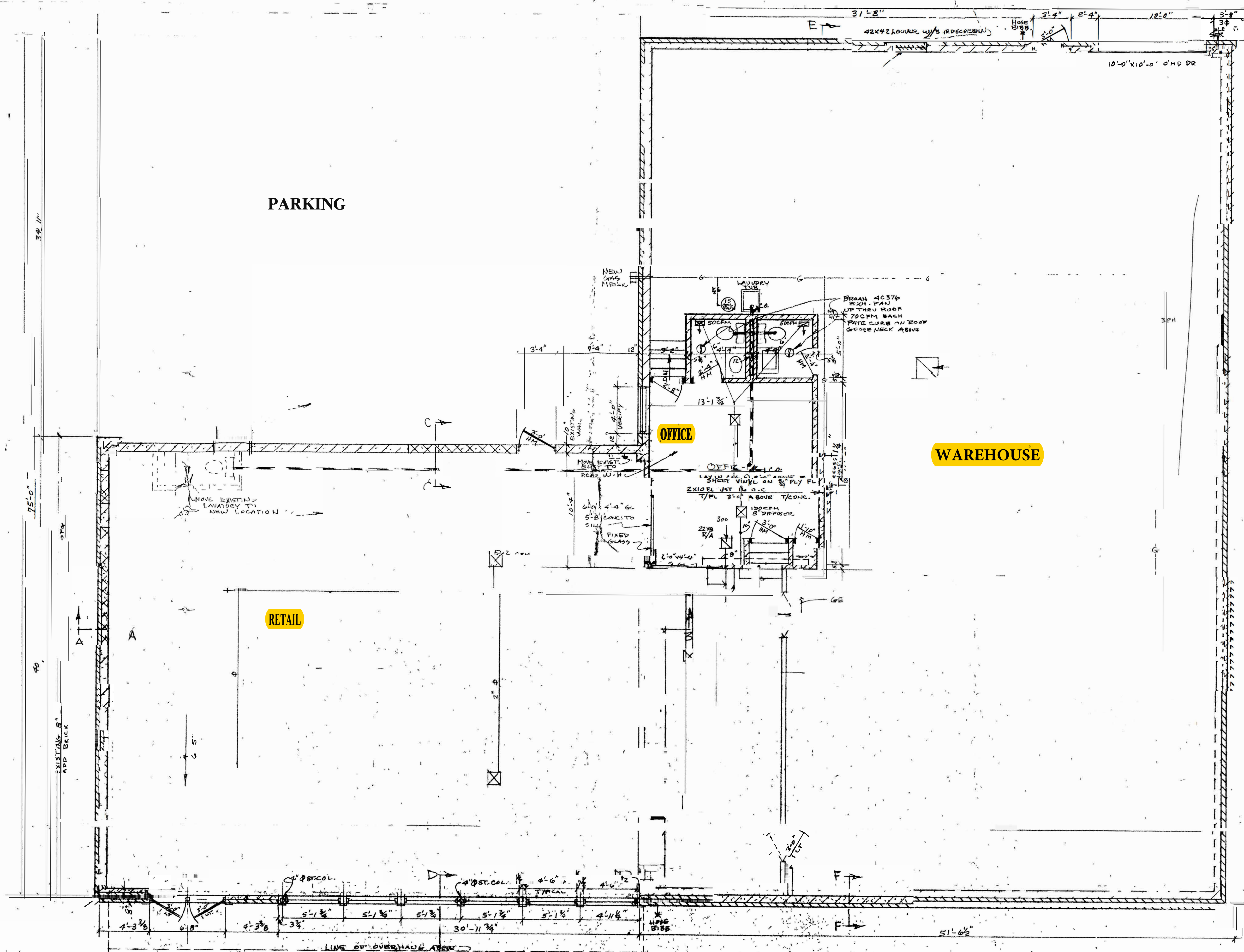
FLOOR PLAN & MECHANICAL LAYOUT SCALE 1/8" = 1'-0"
