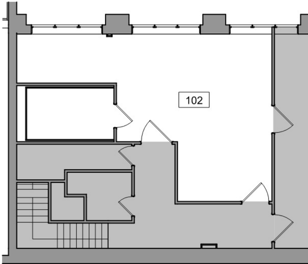
1 Partial Existing Level 3 Floor Plan 1/8" = 1'-0" 4' 8' 16'
