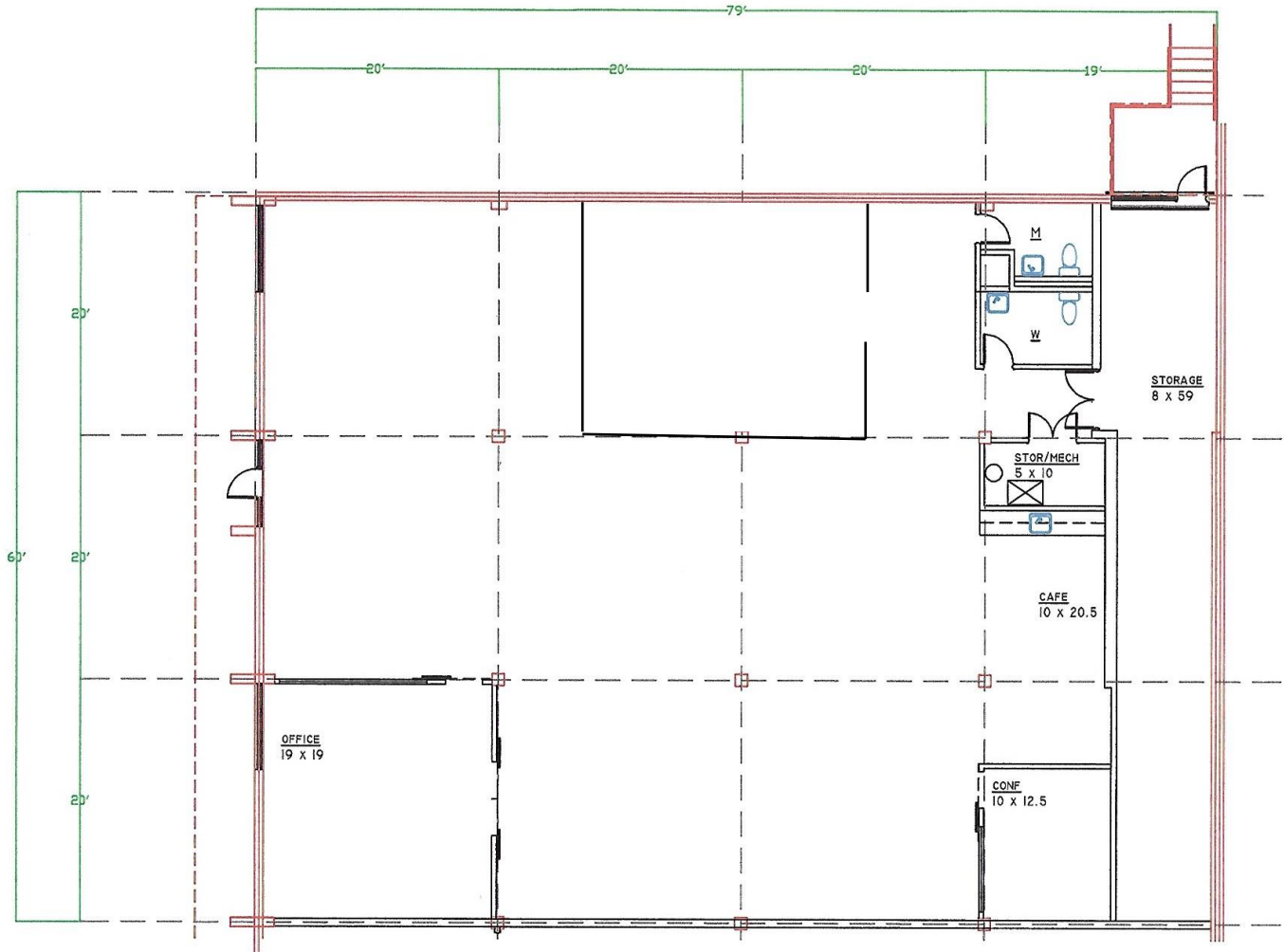
Preliminary Plan #1- Suite E scale \frac{1}{8}''=1'-0''
