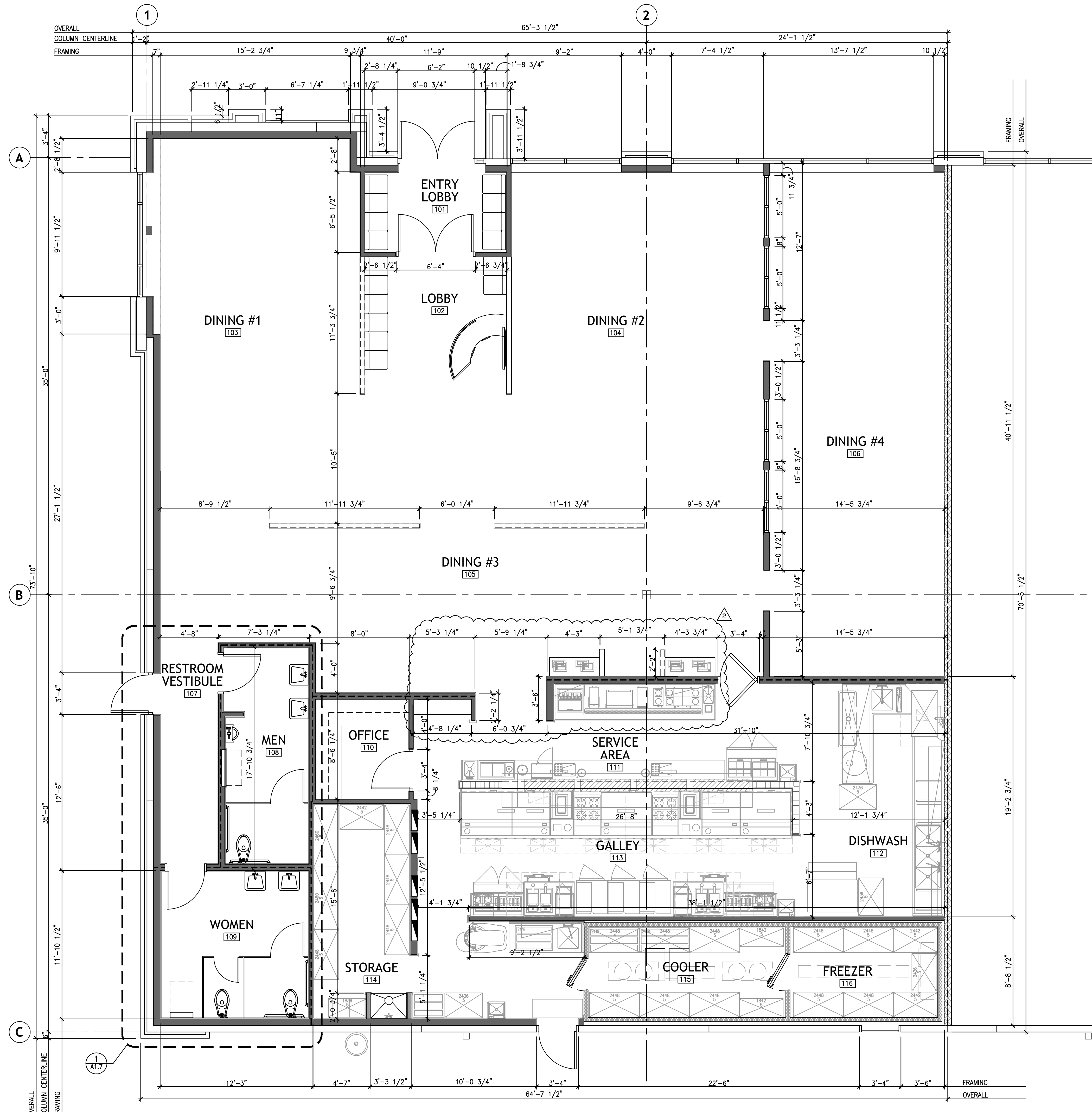
DIMENSIONED FLOOR PLAN 1/4"=1'-0" 1
