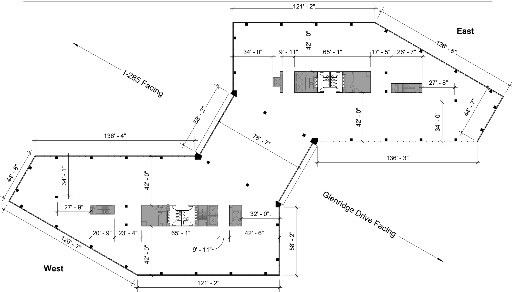
Floor Plan - Suite 300
