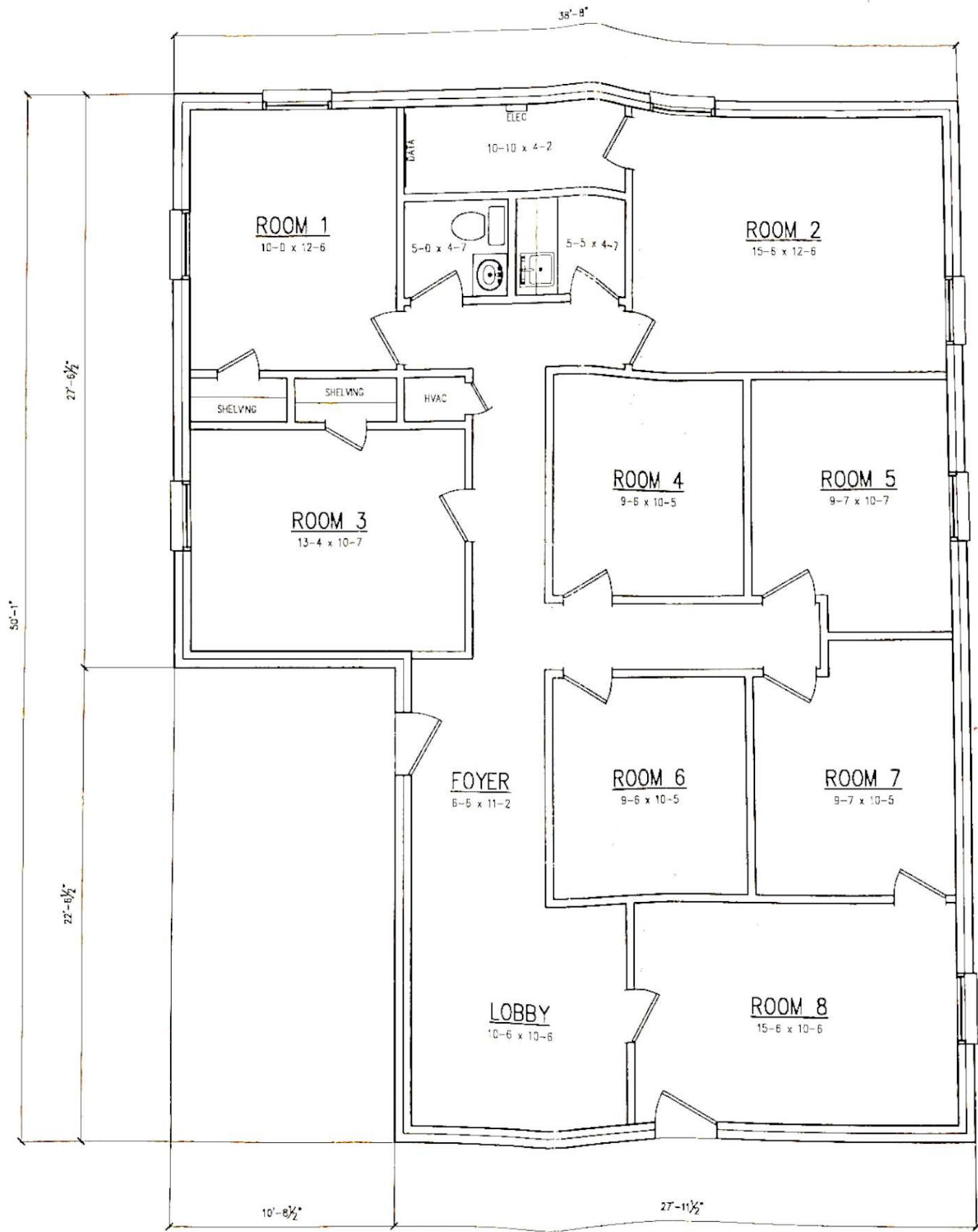
01 FLOOR PLAN A1.0 1/4" = 1'-0"
