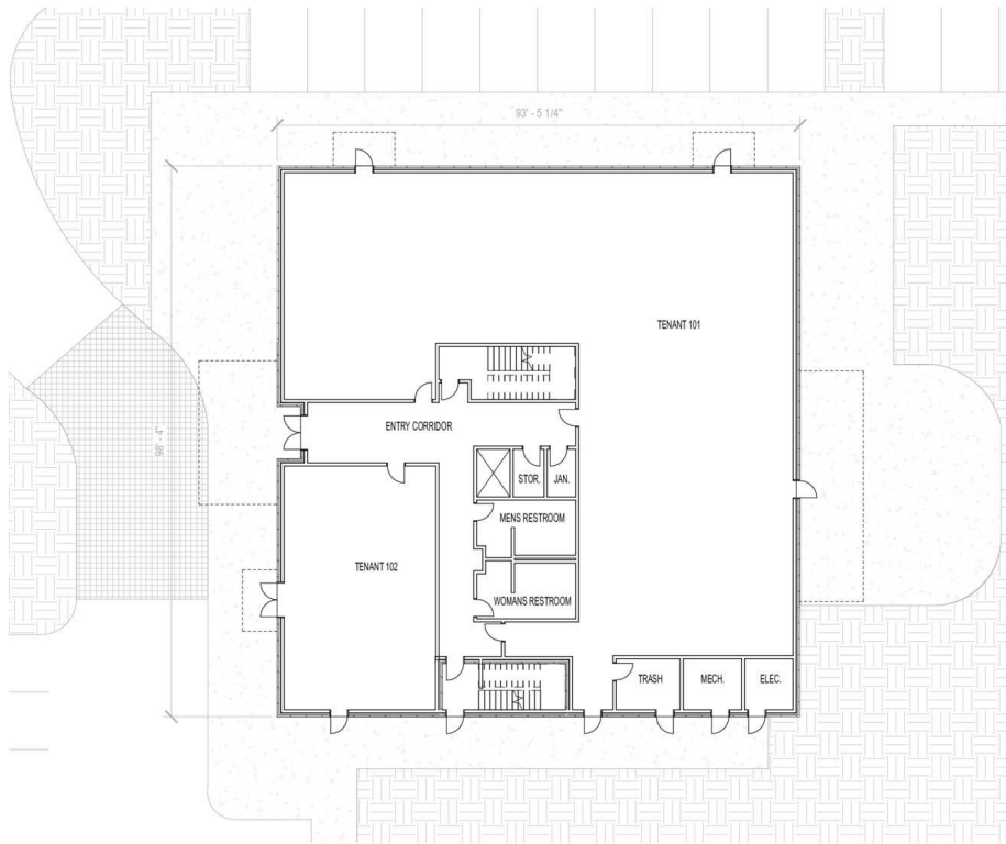
1 FIRST FLOOR PLAN 1/16" = 1'-0"
