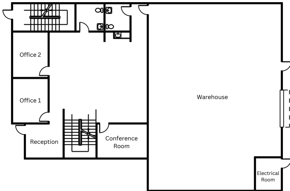
Floor 1
