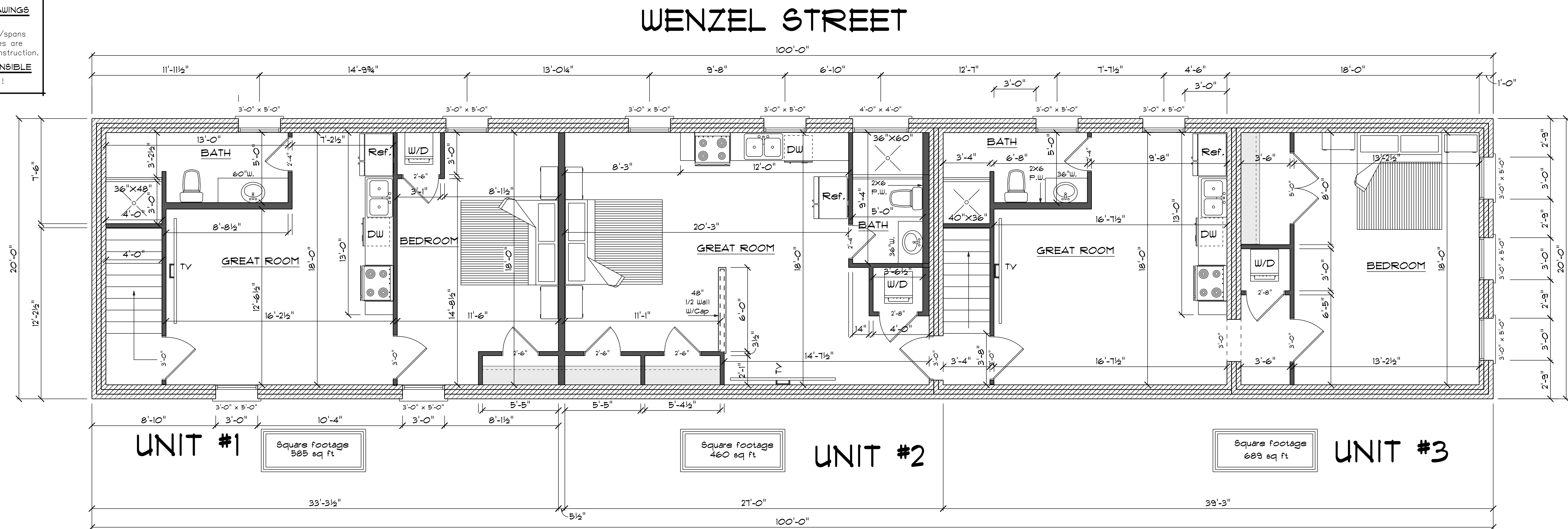
2nd FLOOR PLAN
