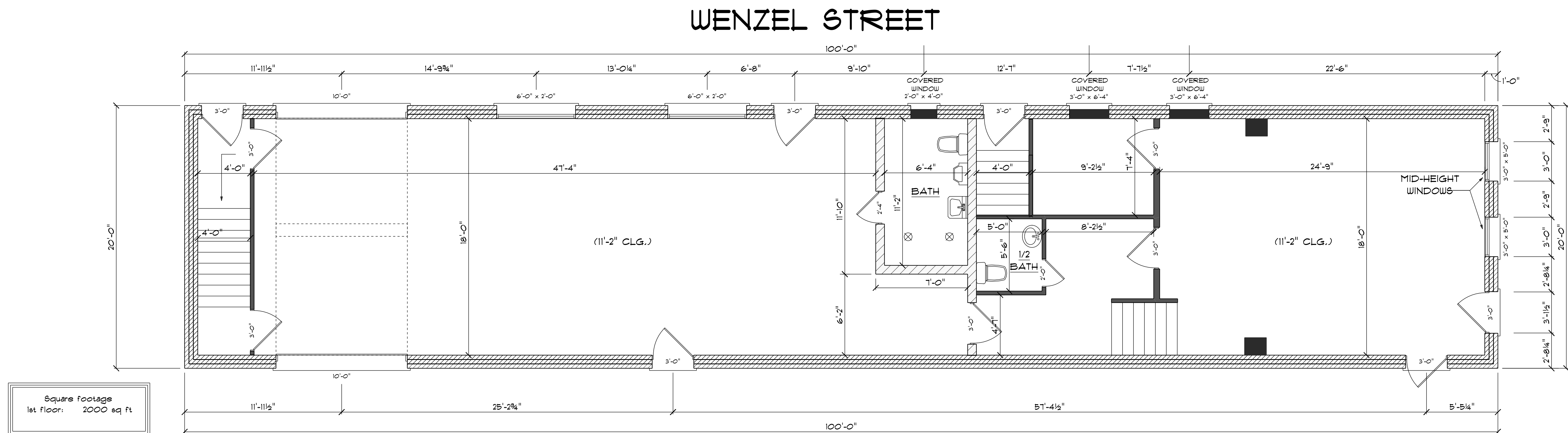
1st FLOOR PLAN
