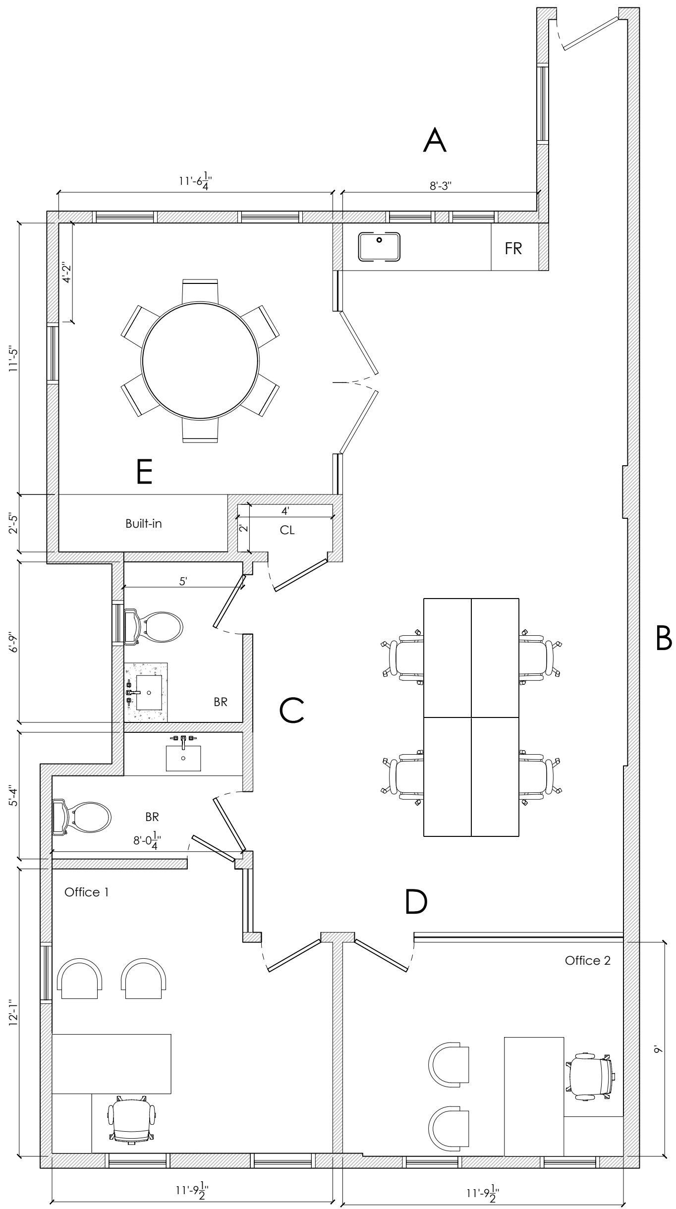
1 PROPOSED FLOOR PLAN Scale: 1/4" = 1'-0"
