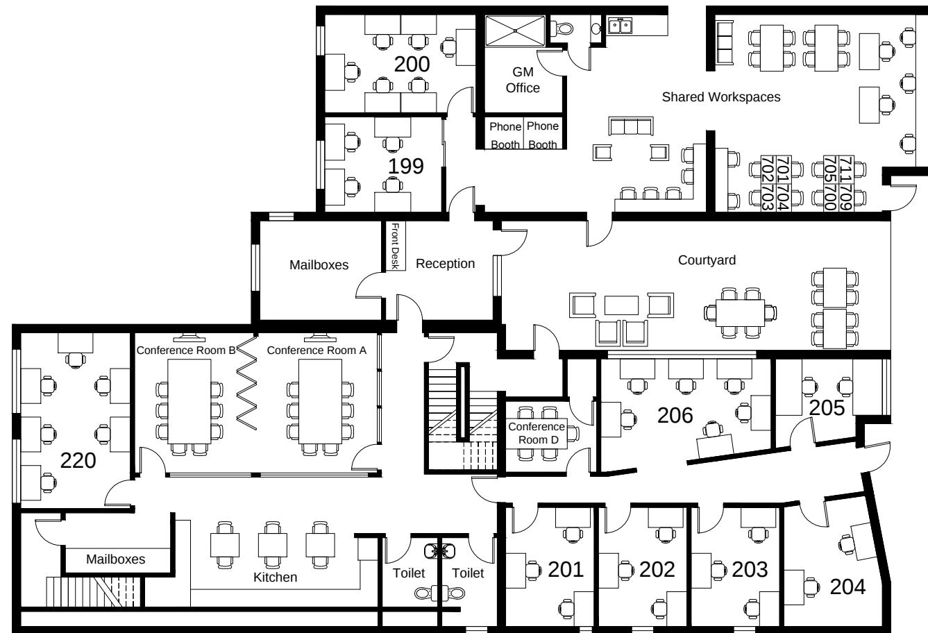
MAIN LEVEL SOUTH WING
