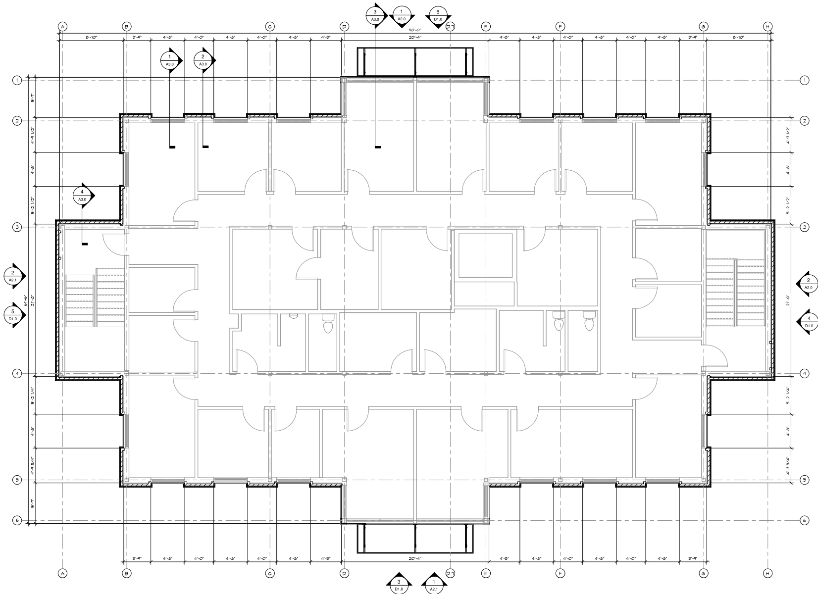
1 SECOND FLOOR PLAN 1/4" = 1'-0"
