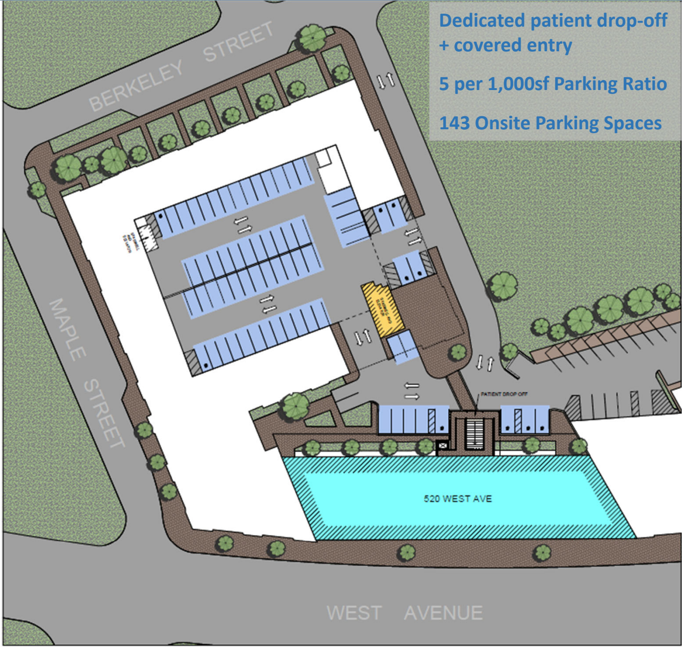
EXISTING SITE AND PARKING LEVEL 1
