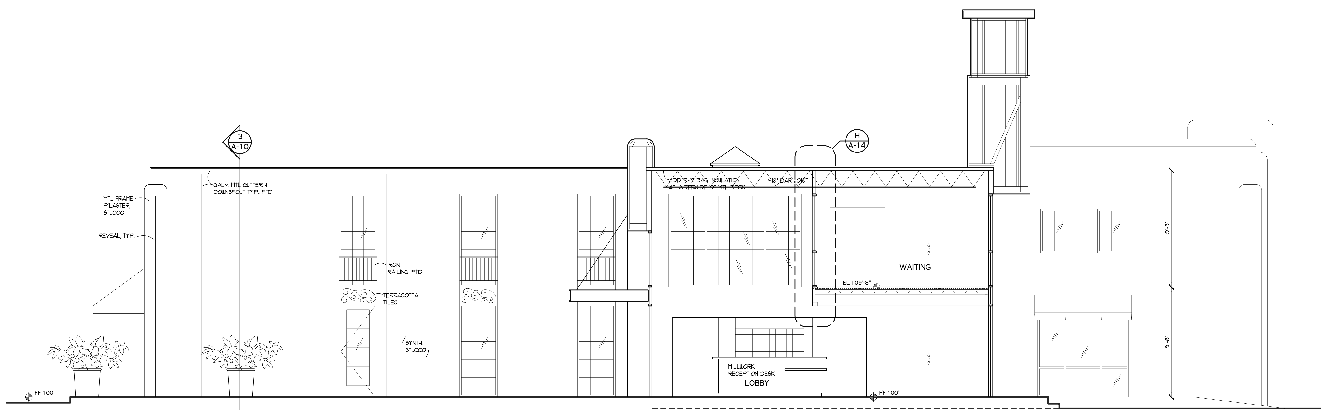
1 NEW LAT. SECT SOUTH SCALE: 1/4" = 1'-0"
