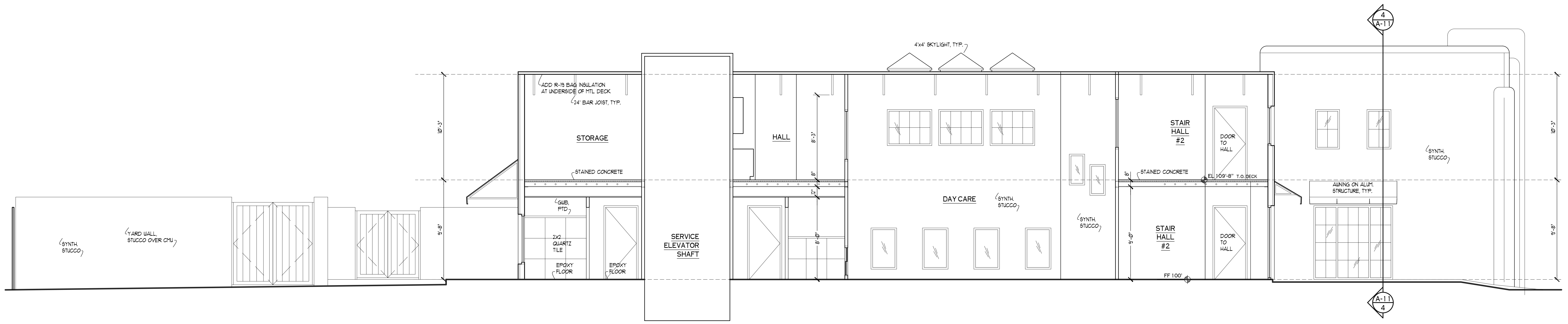
3 NEW LAT. SECT SOUTH SCALE: 1/4" = 1'-0"
