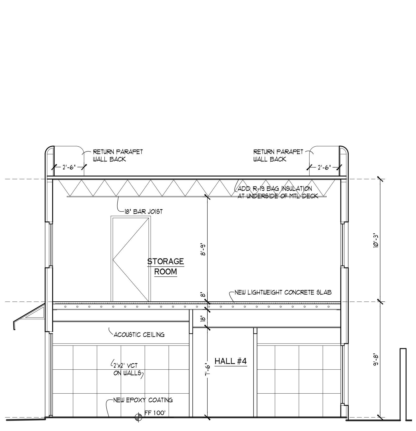
4 NEW SOUTH WING SECTION SCALE: 1/4" = 1'-0"
