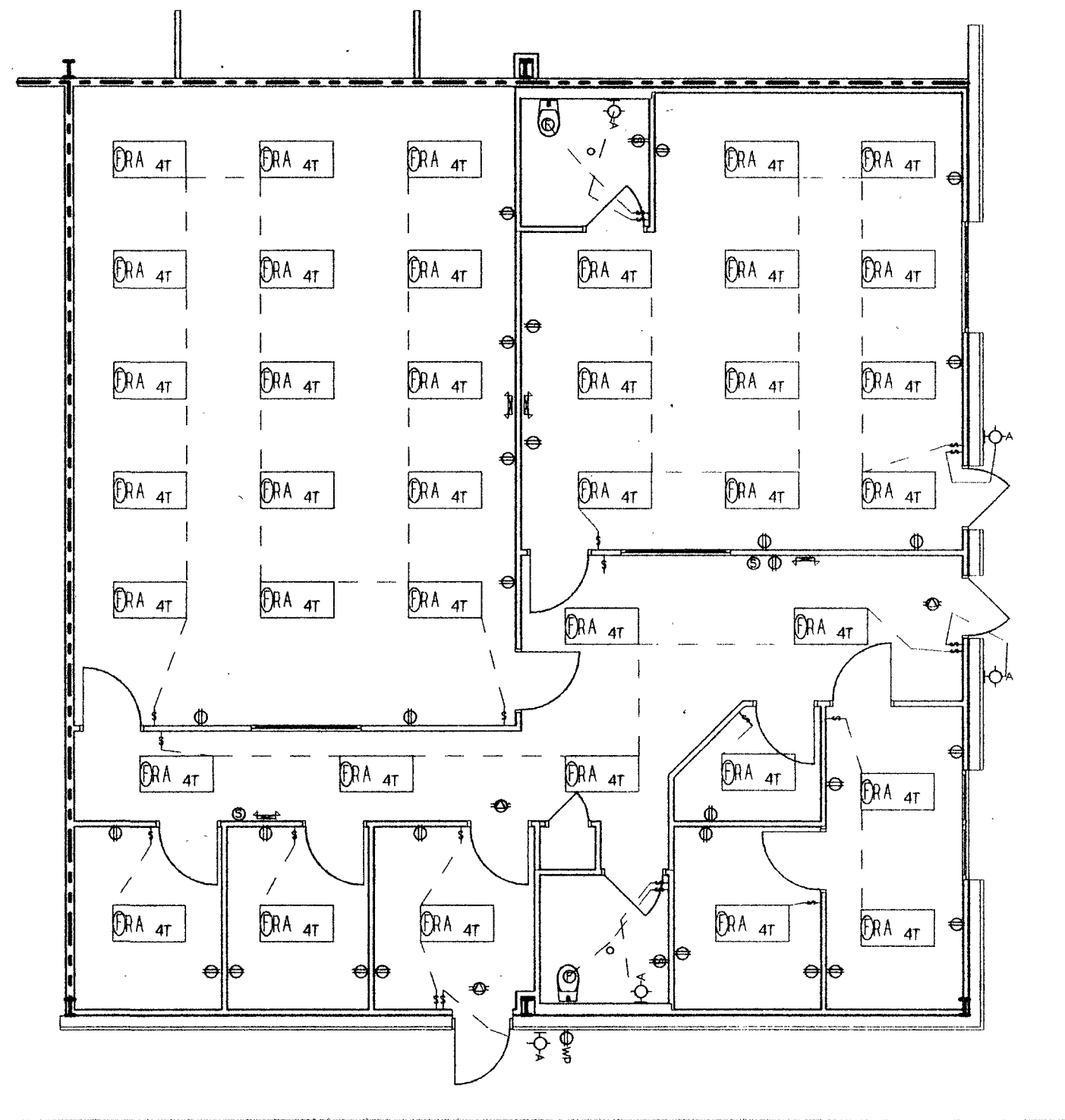
Electrical Layout
