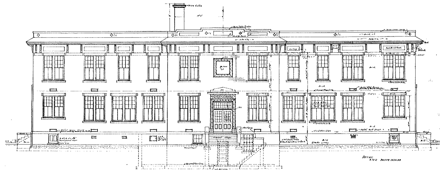
SPENCE AVENUE ELEVATION SCALE 1/8" = 1'-0"
