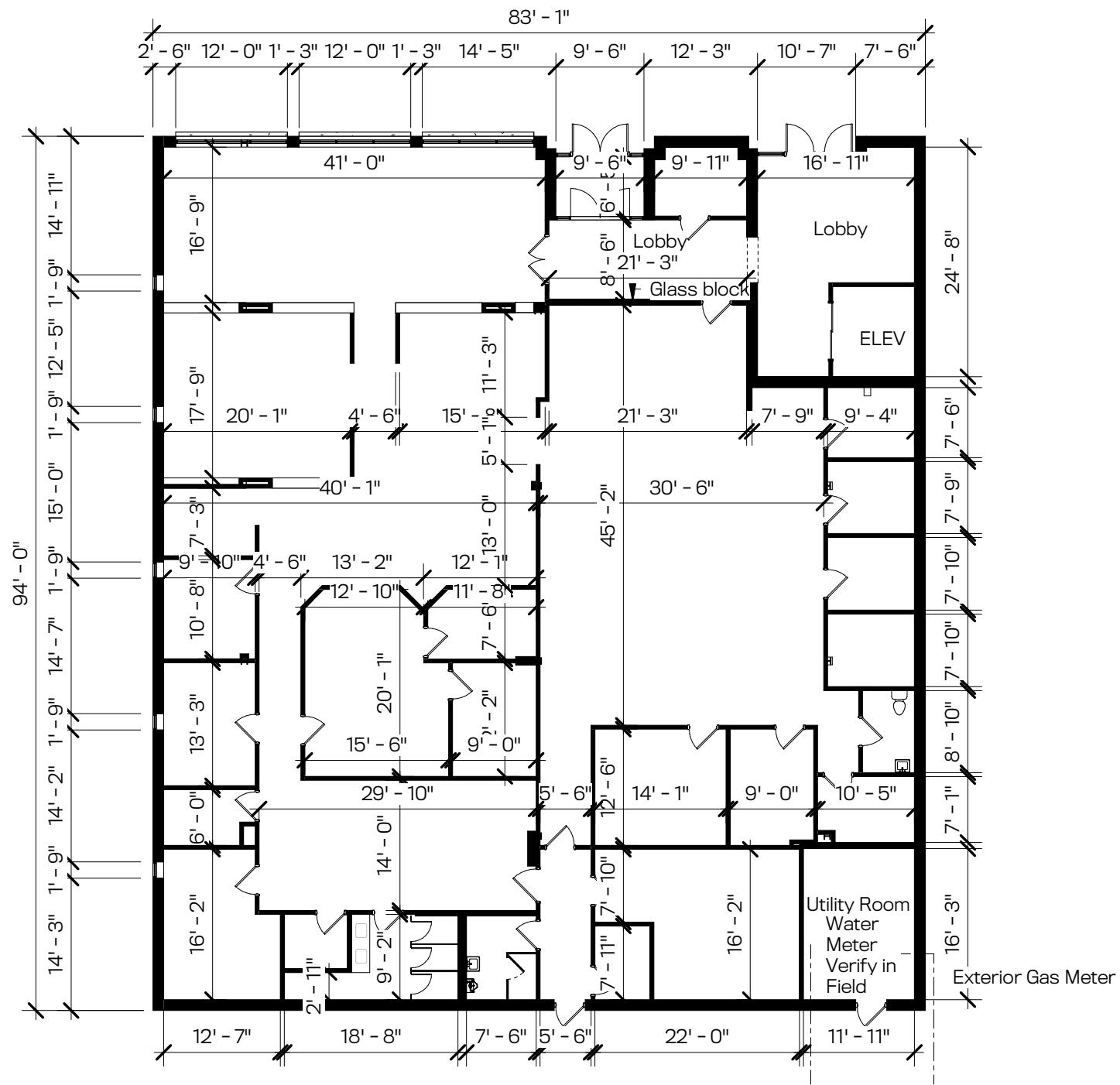
① 01 - First Floor - Existing Area 6994 s.f. 1/16" 1/16" = 1'-0"
