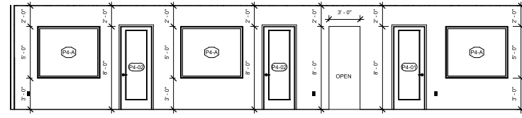
② 210 OFFICES 1/4" = 1'-0"
