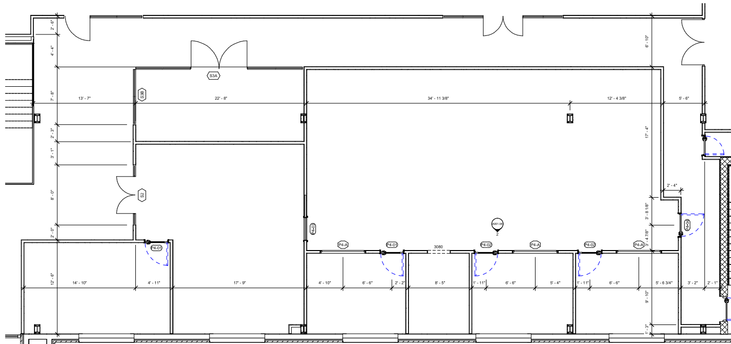
① Phase 4 Framing 1/4" = 1'-0"
