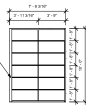
S3B 1/4" = 1'-0"
