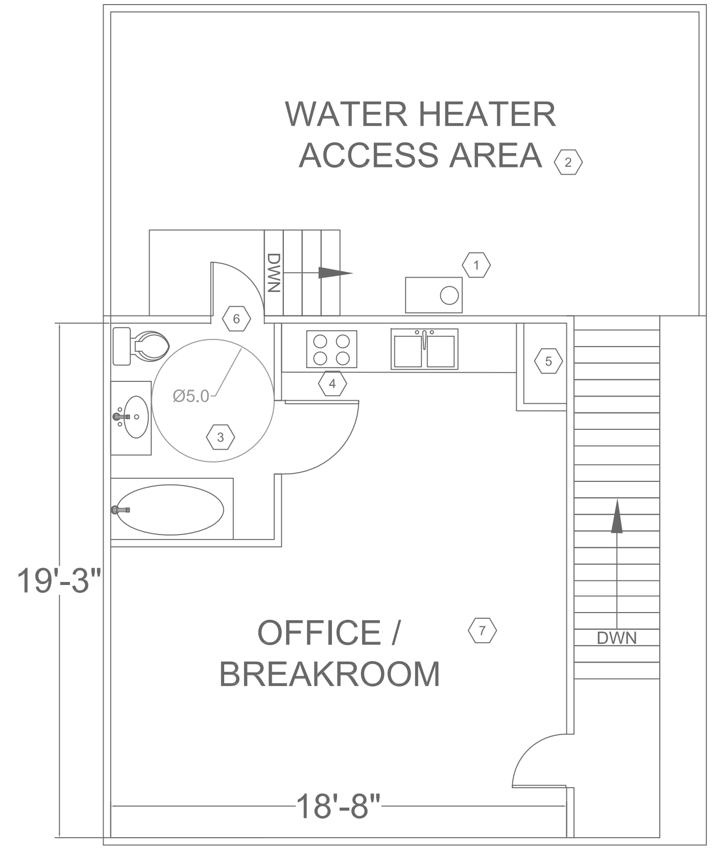
ARCHITECTURAL FLOORPLAN
