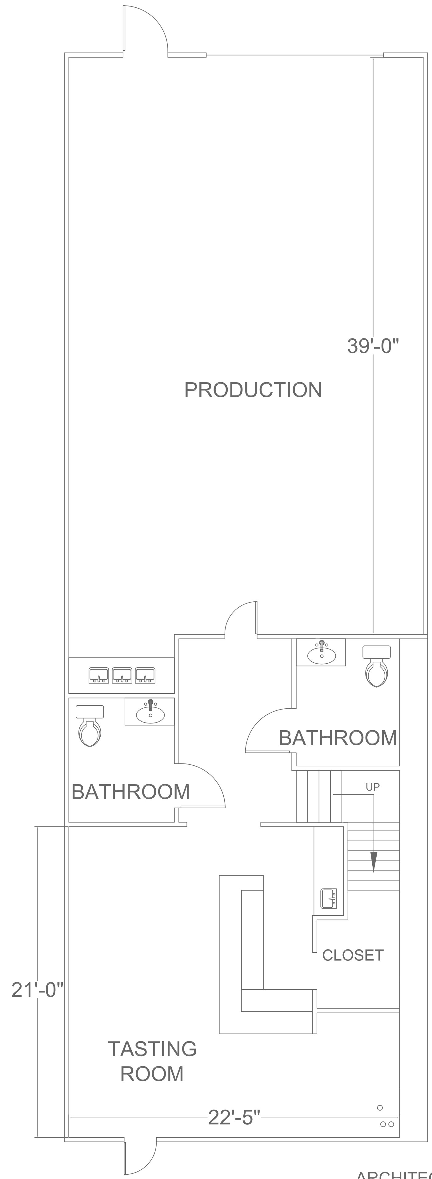
ARCHITECTURAL FLOORPLAN
