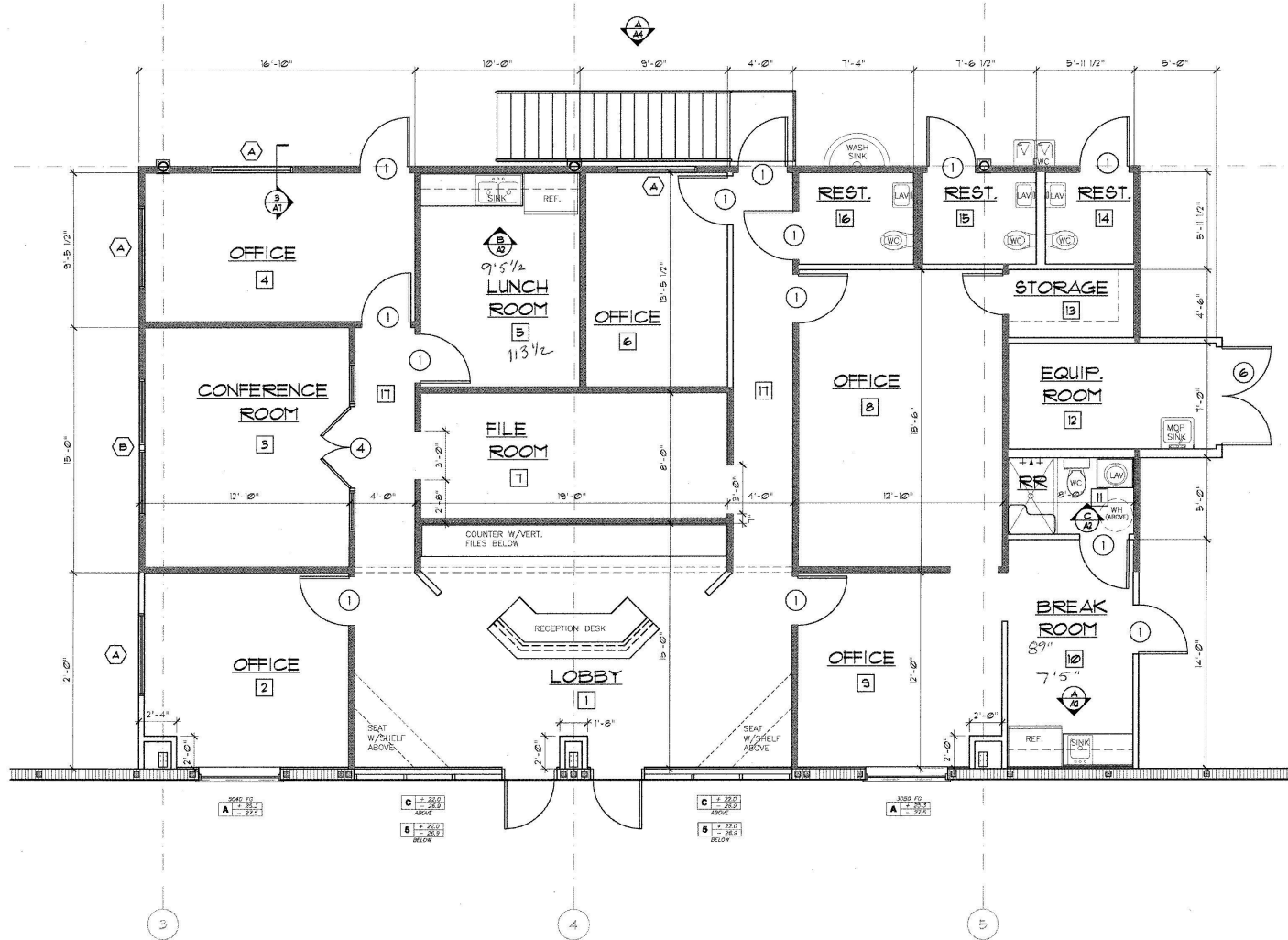
OFFICE FLOOR PLAN 1/4" = 1'-0"
