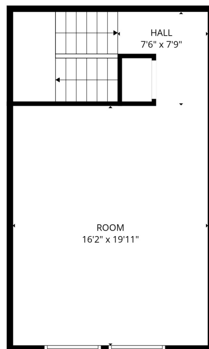
2nd floor
