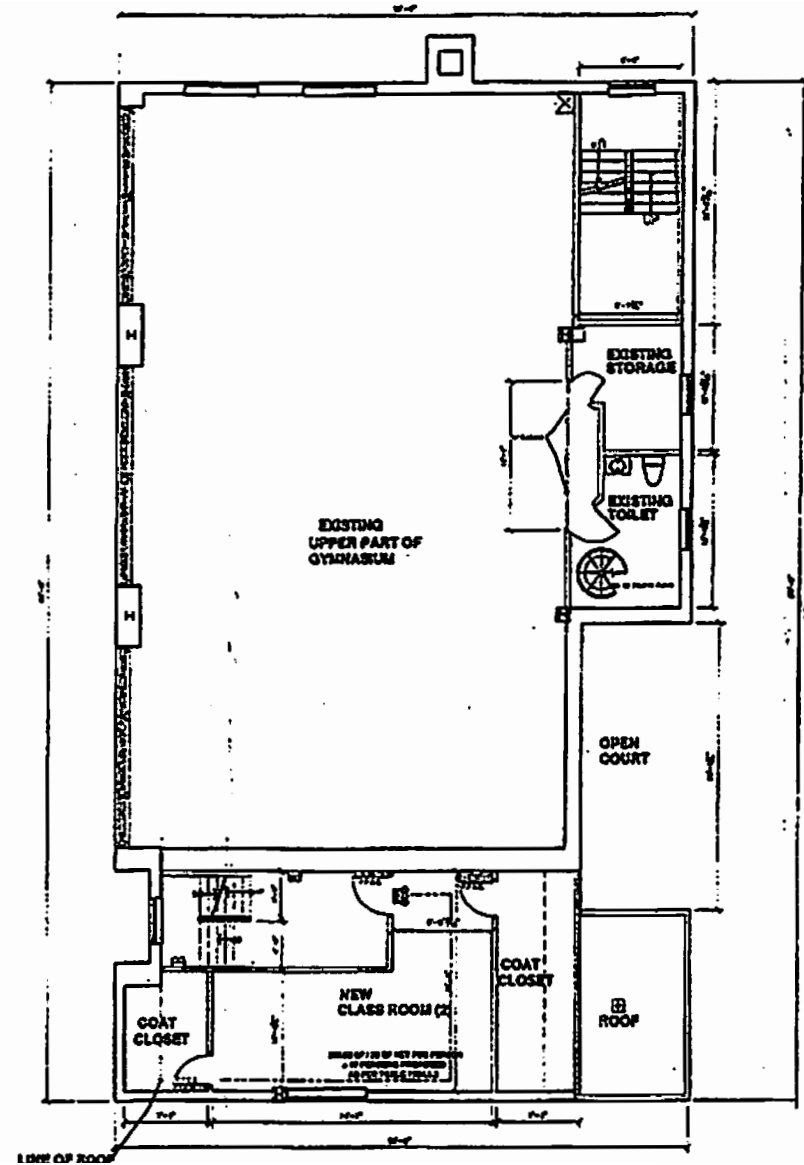
Fourth Floor Mezzanine
