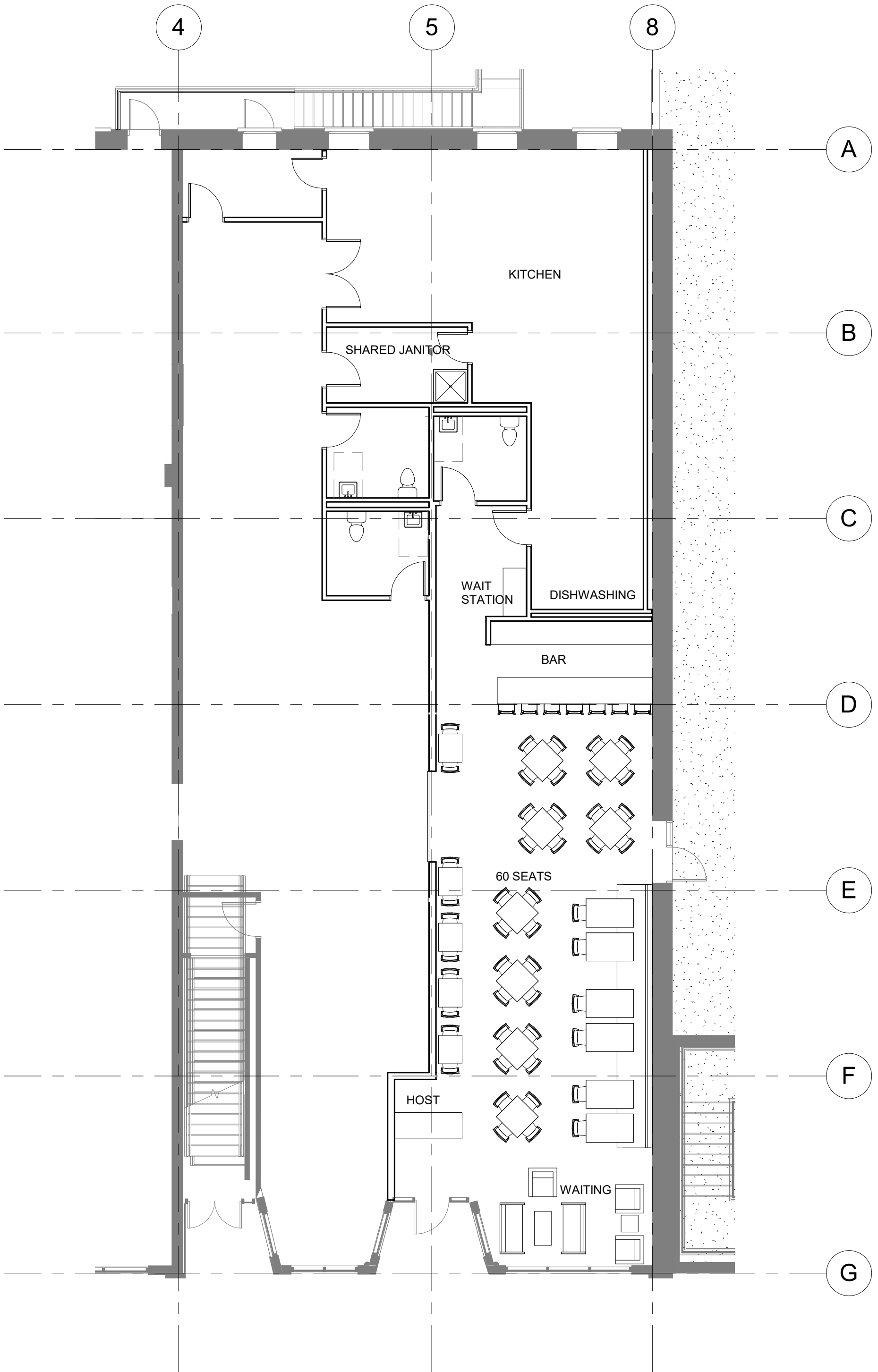
1 LEVEL 1 RESTAURANT OPTION A 1/8" = 1'-0"
