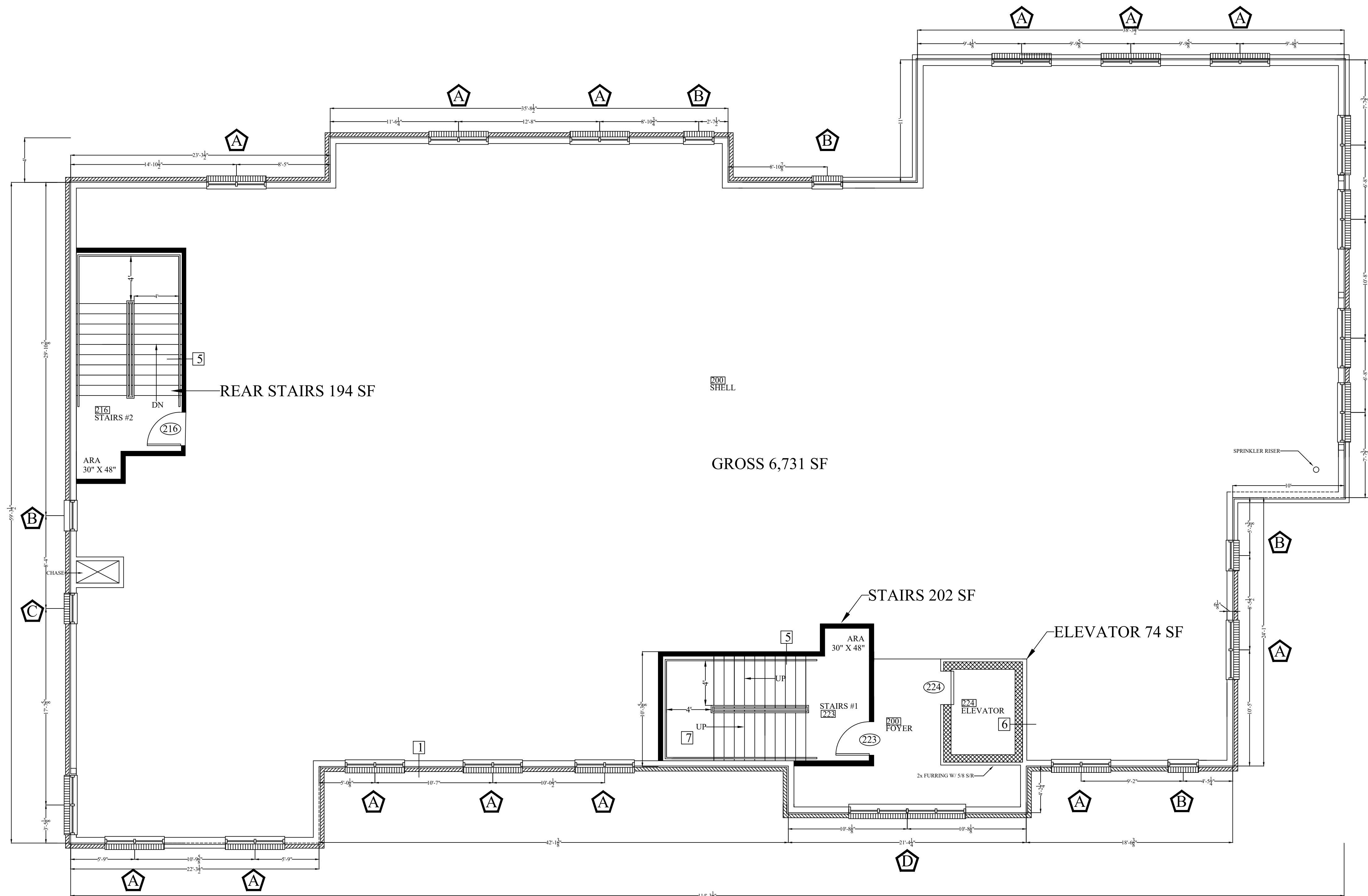
1 2ND FLOOR PLAN G102 3/16" = 1'0"
