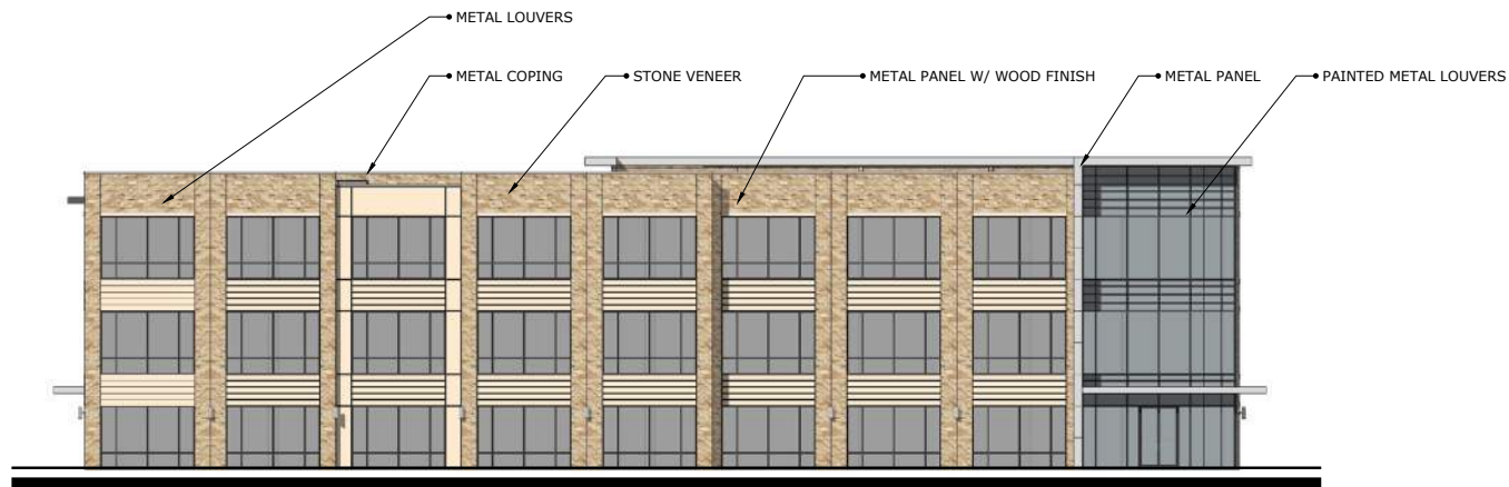
West Elevation
