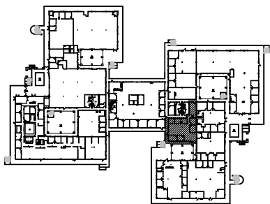
SECOND FLOOR OVERALL PLAN
