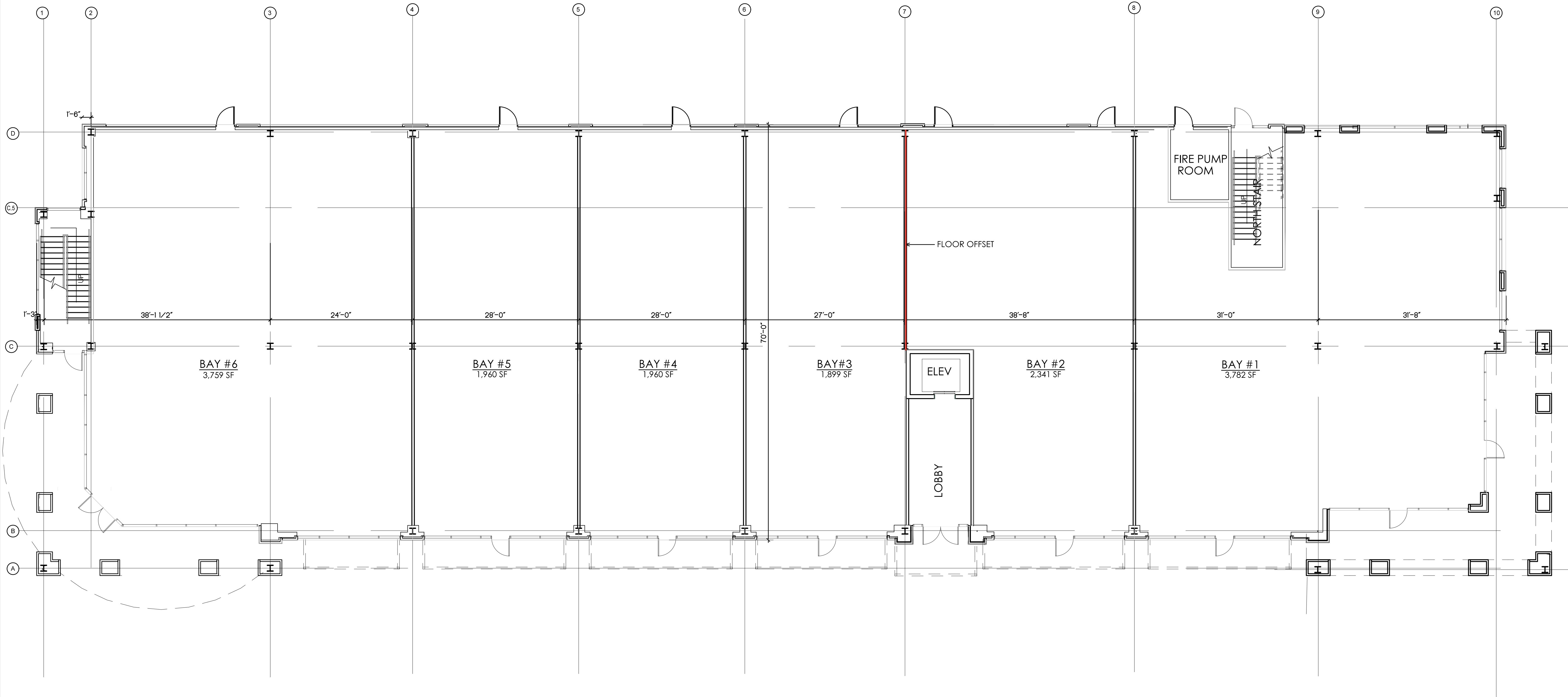
FIRST FLOOR PLAN SCALE: 1/8" = 1'-0"
