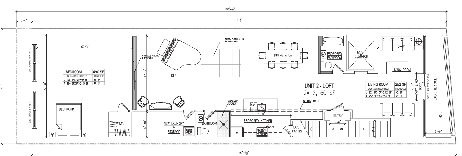
2ND FLOOR
