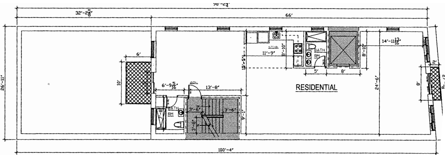
6TH FLOOR
