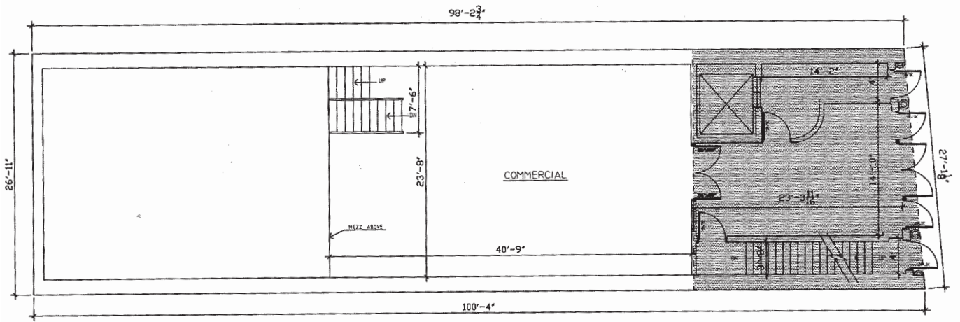
GROUND FLOOR
