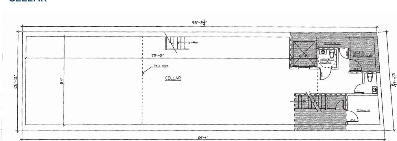
CELLAR
