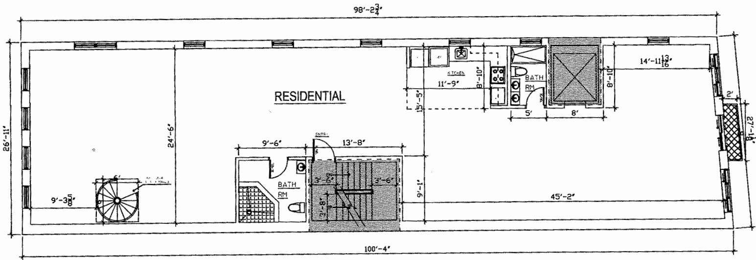
4TH FLOOR
