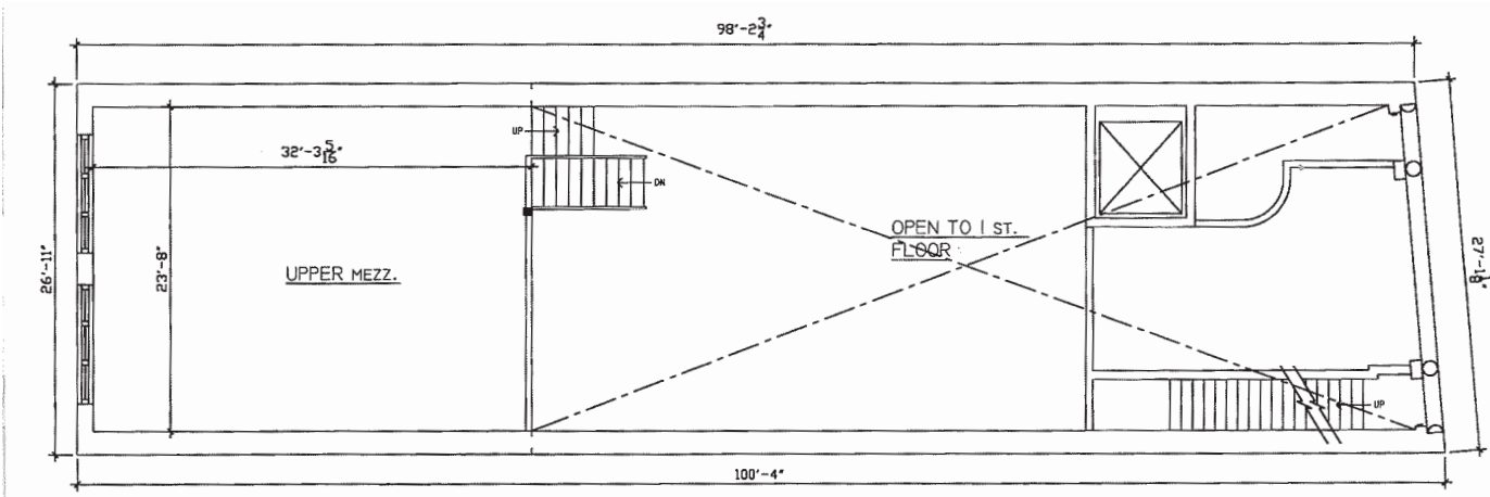
MEZZANINE
