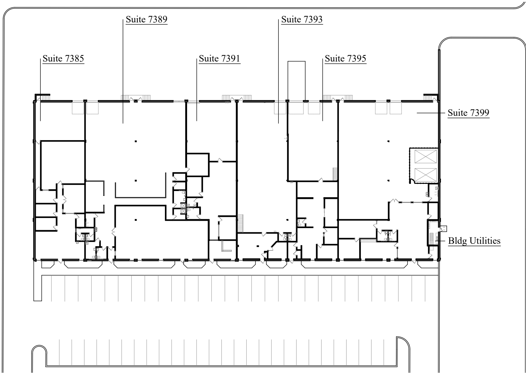
Full Building Plan Scale: 1" = 40'-0"
