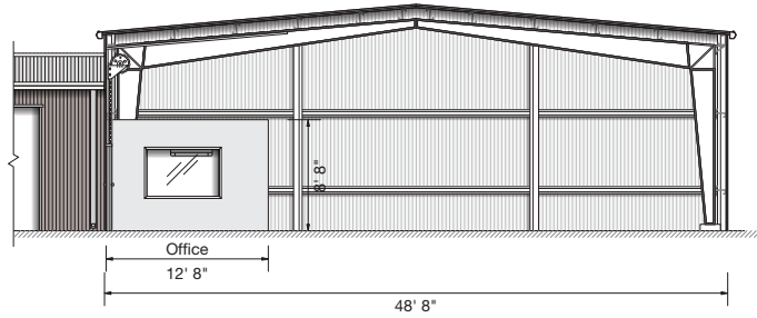
Site Elevation (Northside)
