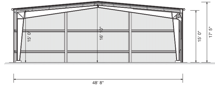
Site Elevation (Southside)
